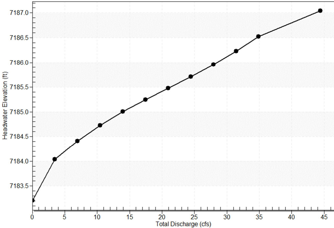
Total Rating Curve Crossing: G1 Pond Culvert
