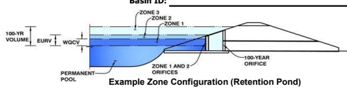
Example Zone Configuration (Retention Pond)
