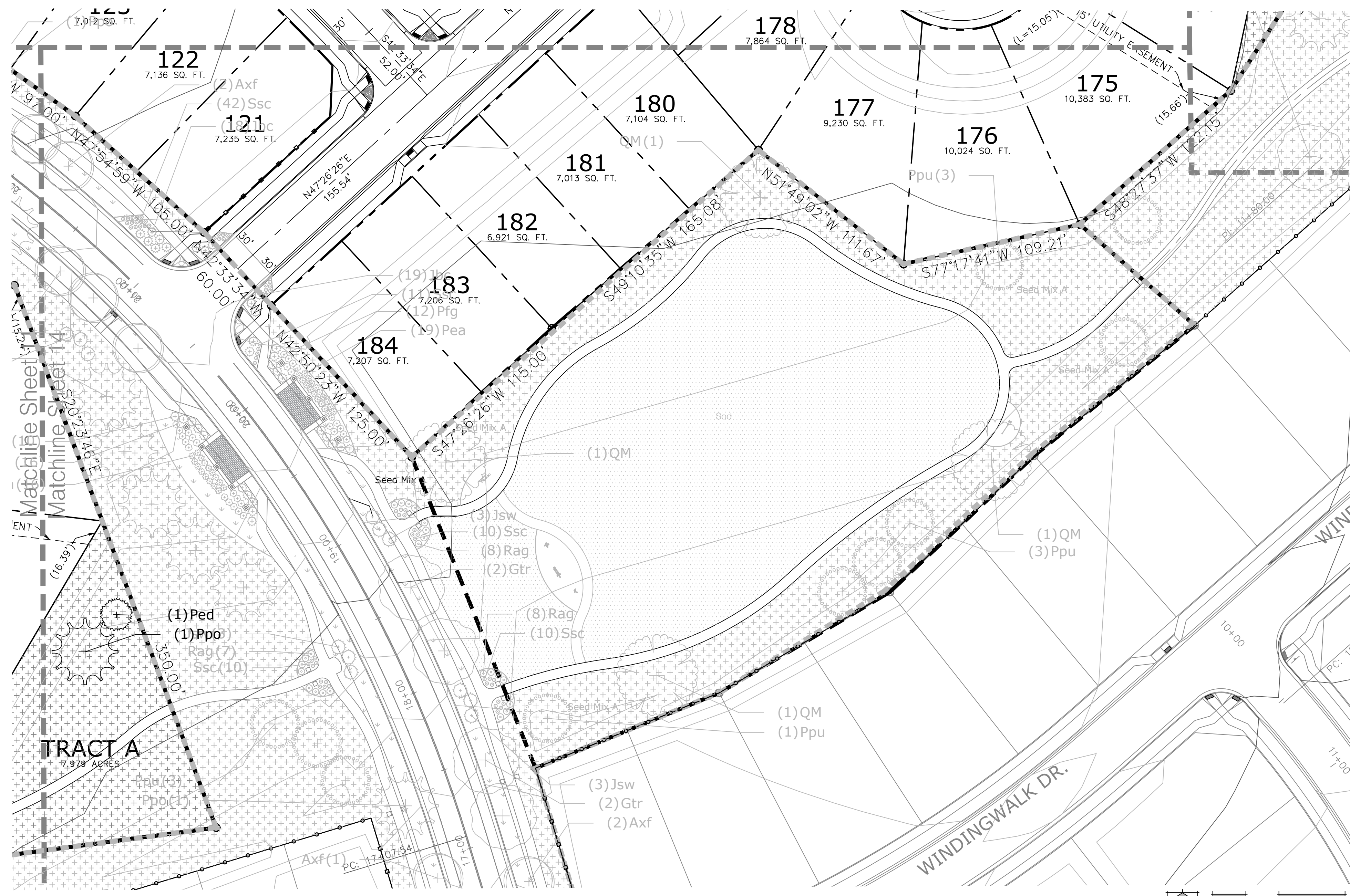
14 LANDSCAPE PLAN
