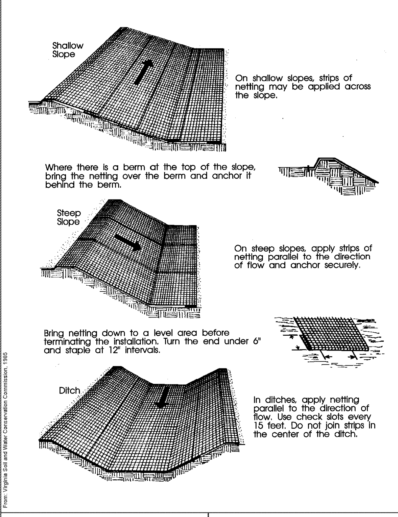
City of Colorado Springs Storm Water Quality Figure ECB-2 Erosion Control Blanket Installation Requirements DENM153722.CS.CDF/gcib-25-99
