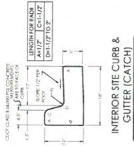
INTERIOR SITE CURB & GUTTER (SPILL) SCALE: 1/4" = 1'-0"
