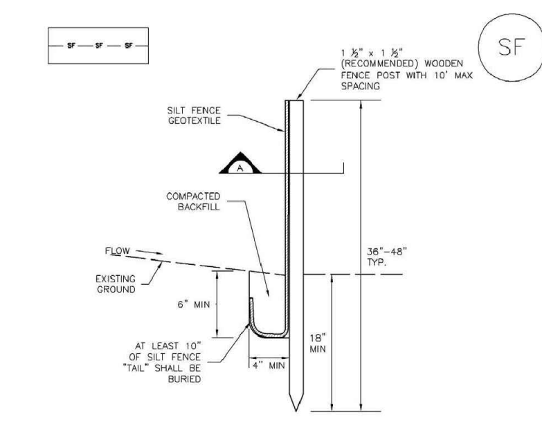
SILT FENCE
