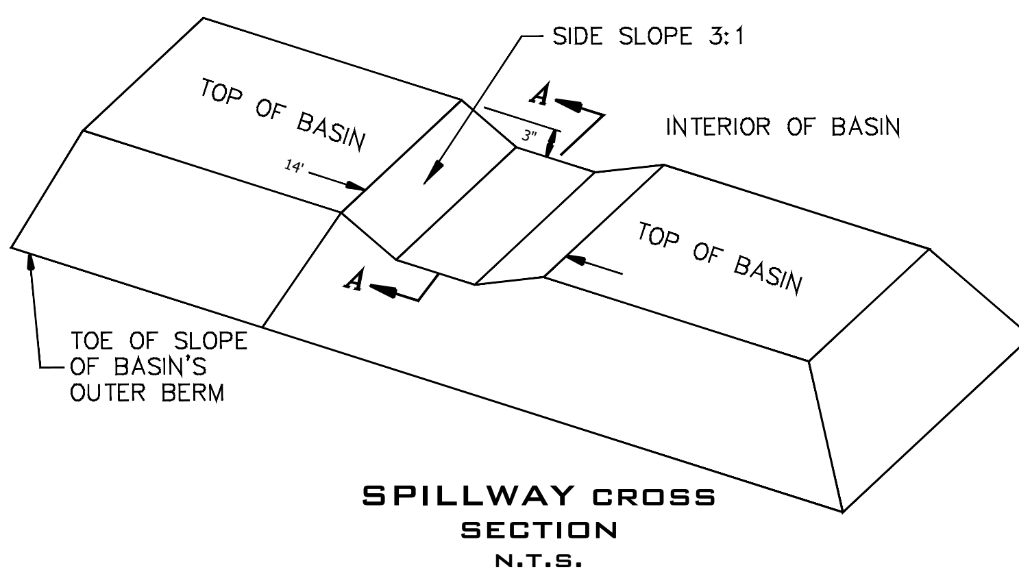
SECTION: A-A
