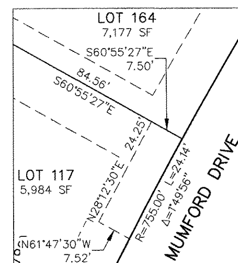
MAIL KIOSK EASEMENT DETAIL
