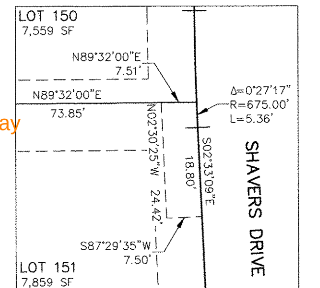
MAIL KIOSK EASEMENT DETAIL
