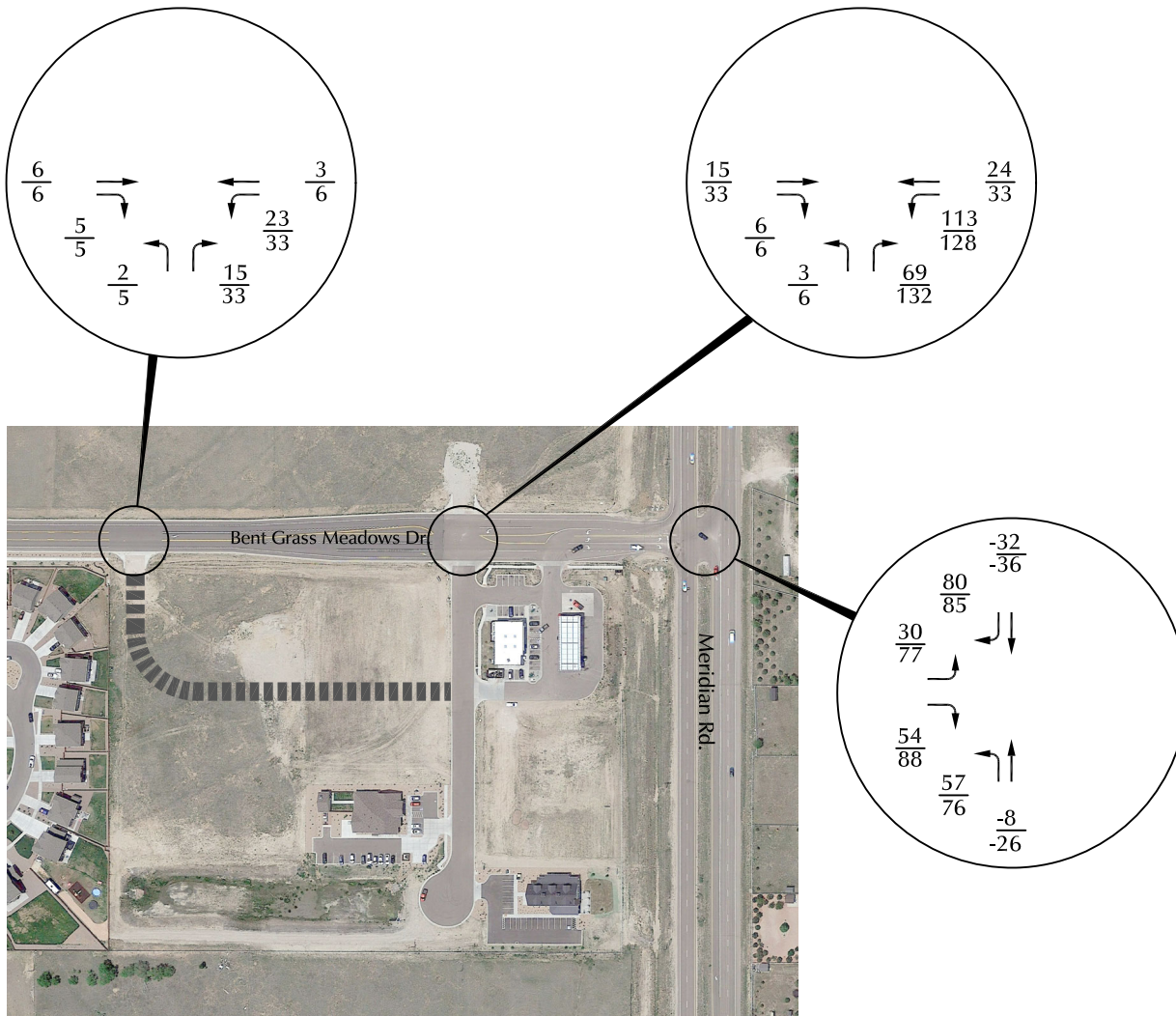
Figure 9 Assignment of Future Site-Generated Traffic (TAZ 8 & 9) Bent Grass Meadows (LSC #194900)
