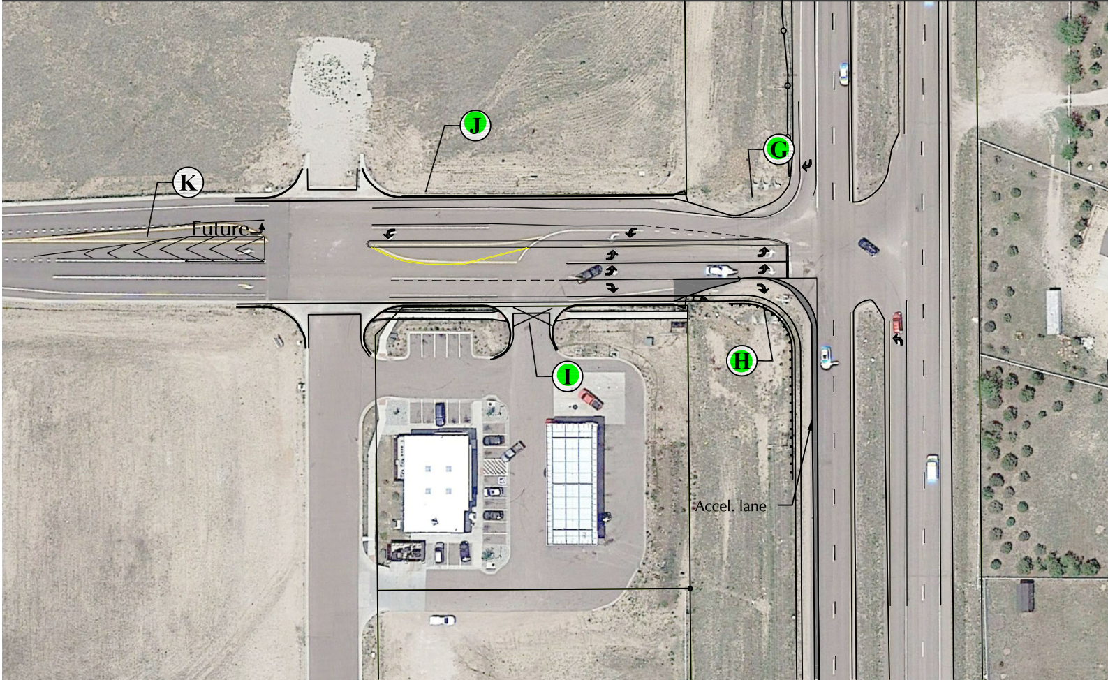
Figure 12 Future Roadway Improvements Bent Grass Meadows (LSC #194900)
