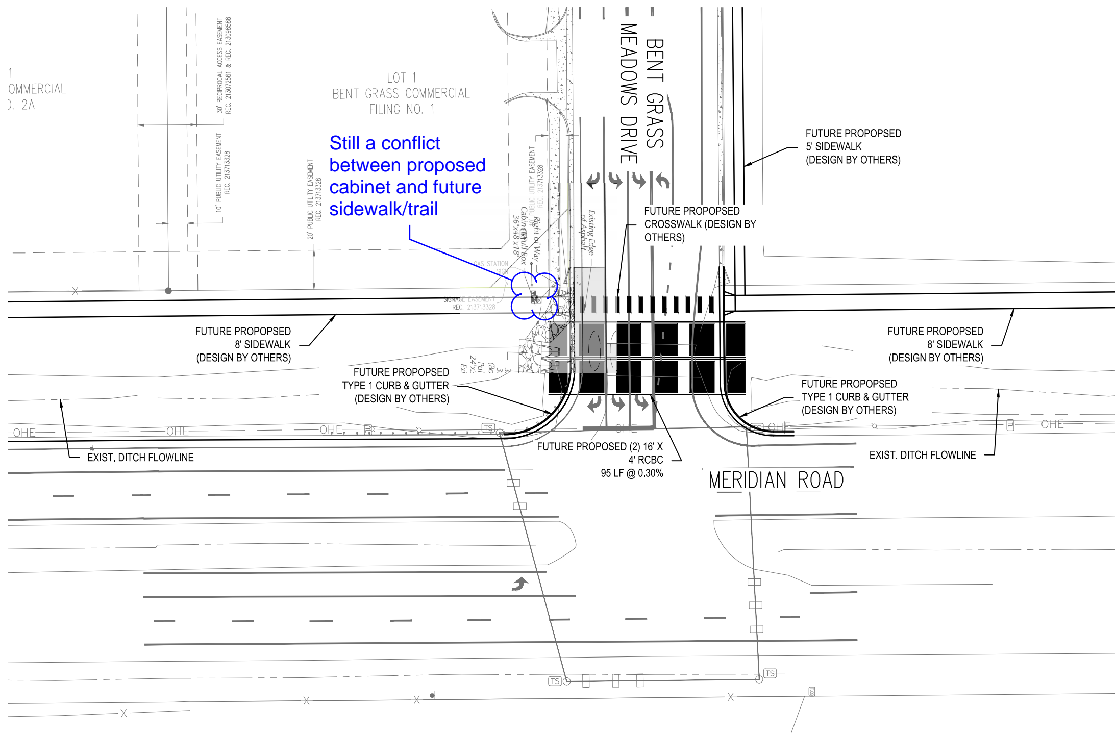
FUTURE PROPOSED SIDEWALK SCALE: 1"=50'
