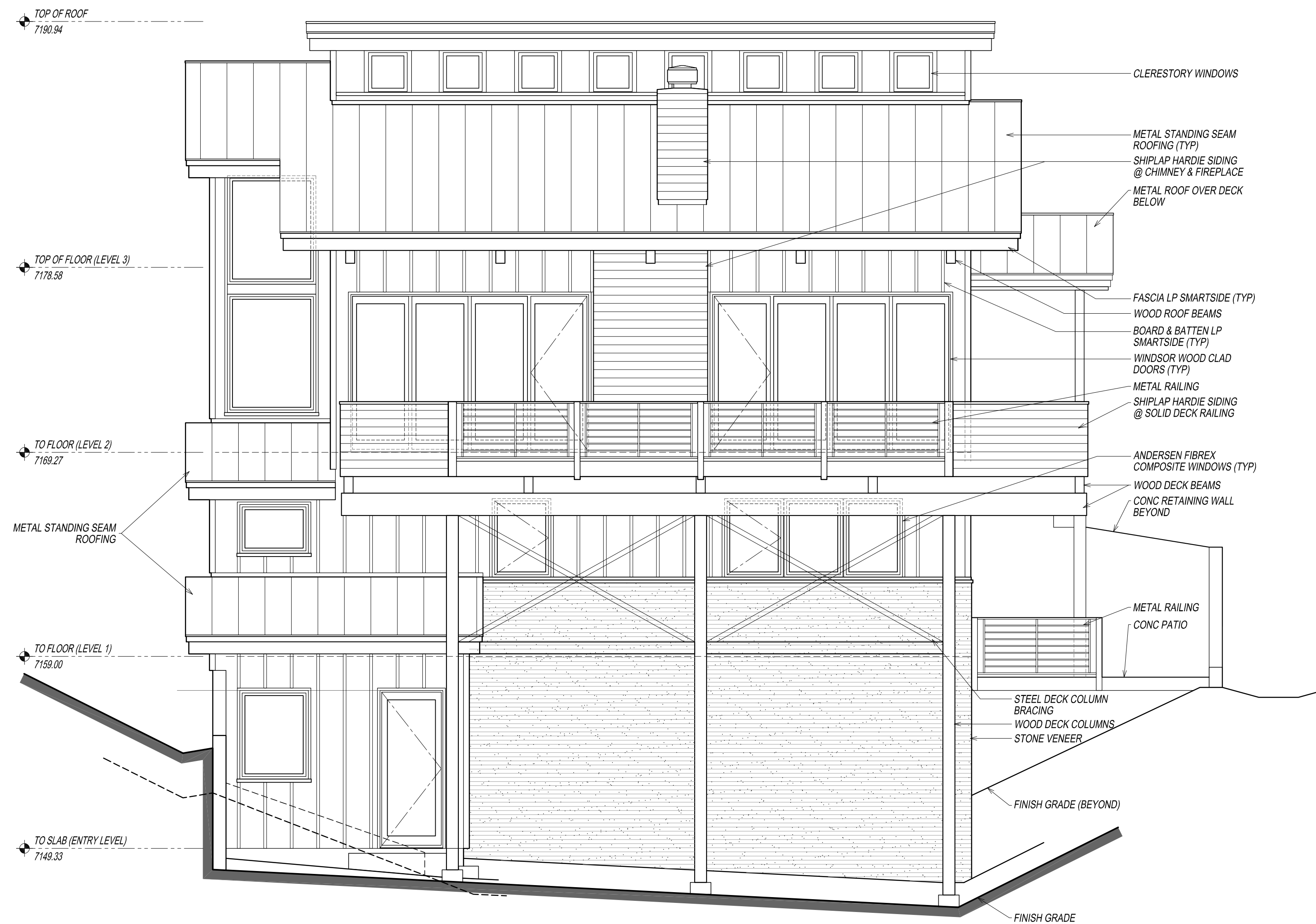
20 WEST BUILDING ELEVATION SCALE: 1/4"=1'-0"
