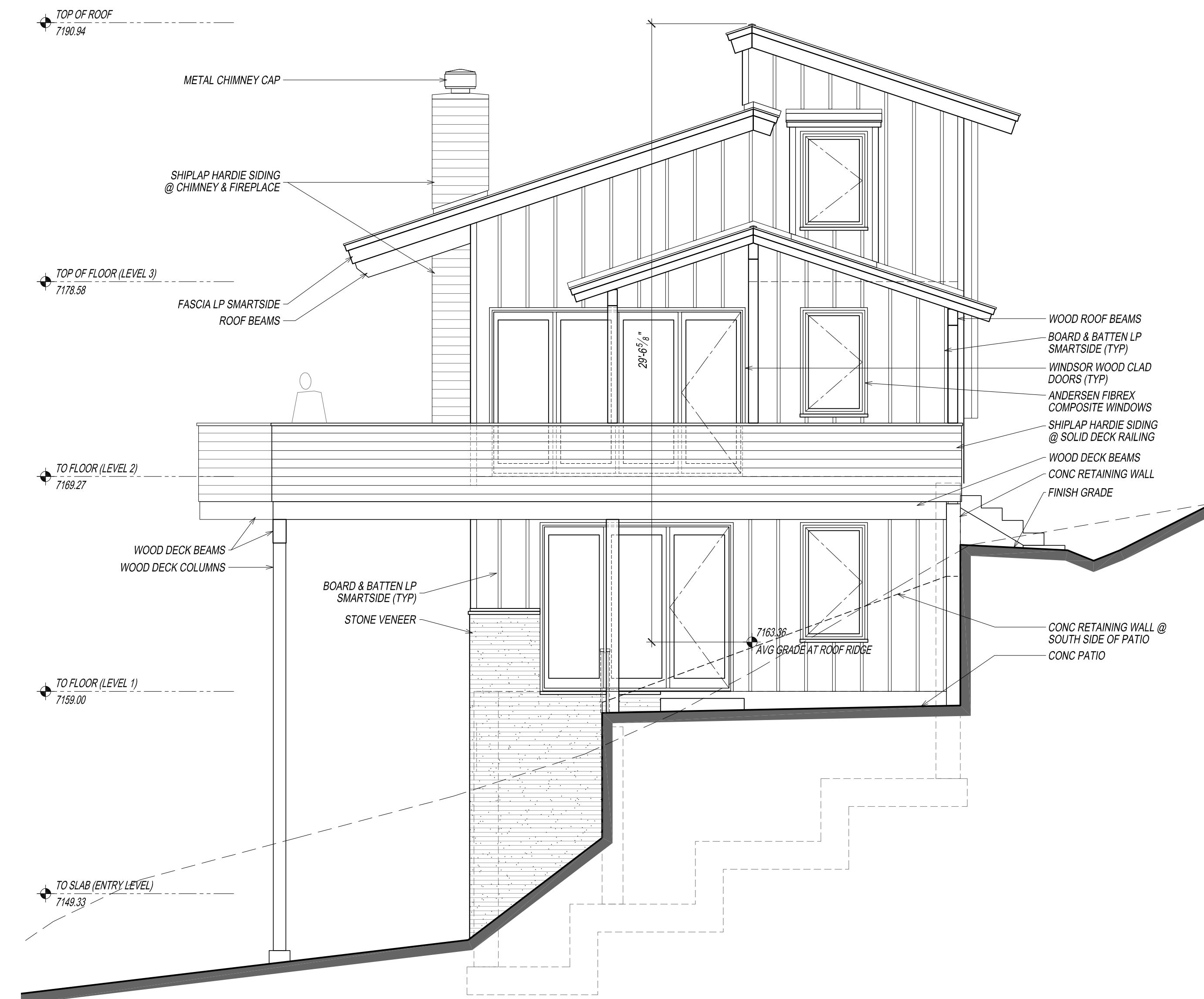
23 SOUTH BUILDING ELEVATION SCALE: 1/4"=1'-0"
