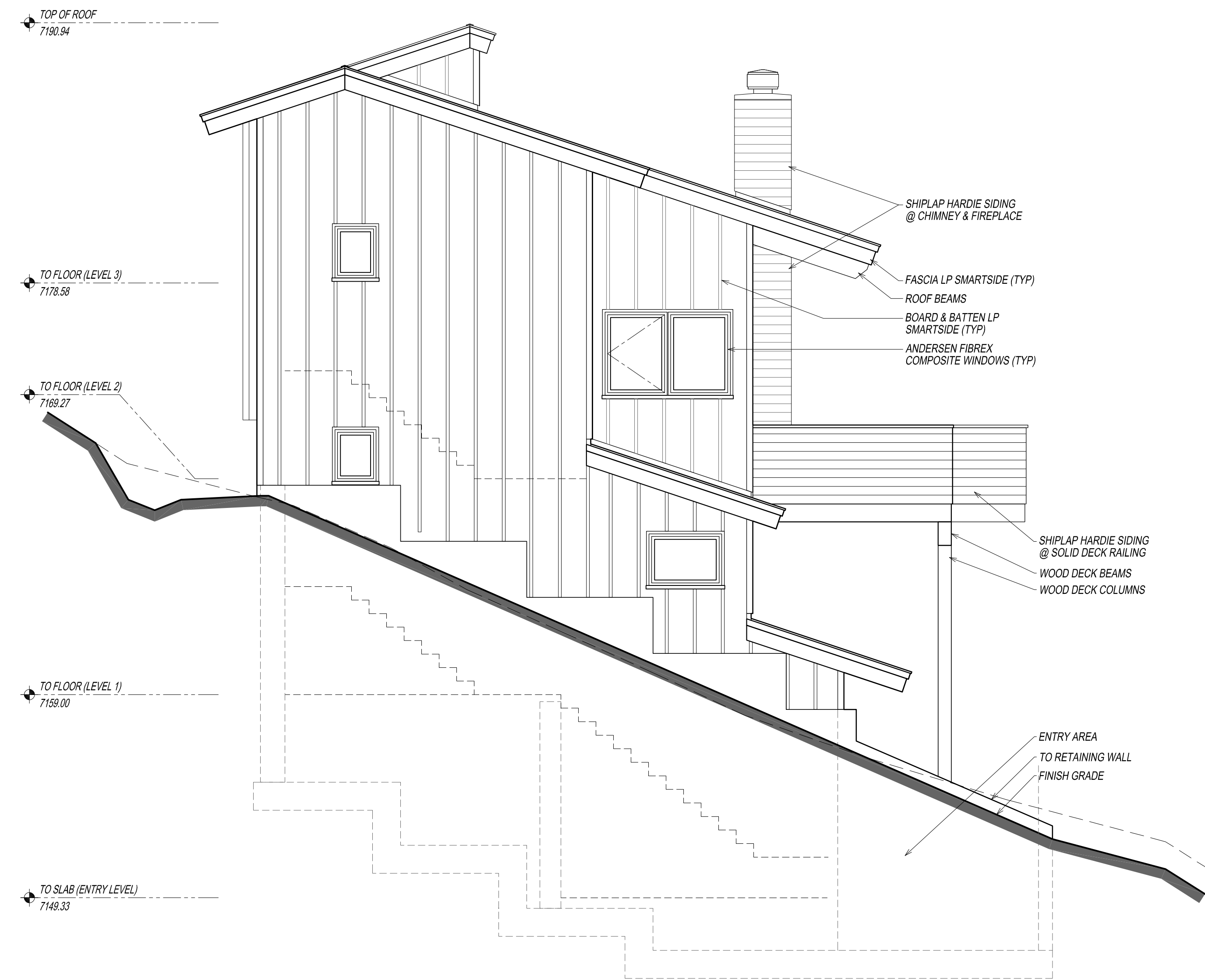
23 NORTH BUILDING ELEVATION SCALE: 1/4"=1'-0"
