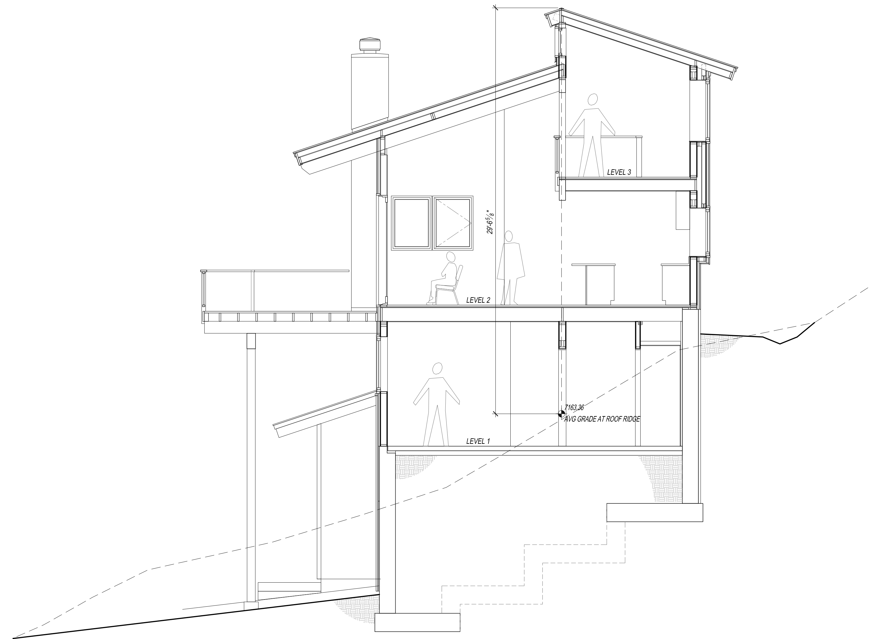
BUILDING SECTION SCALE: 1/4"=1'-0"
