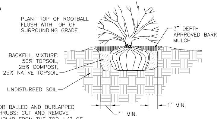
B SHRUB/DECORATIVE GRASS PLANTING LS2 SCALE: N.T.S.
