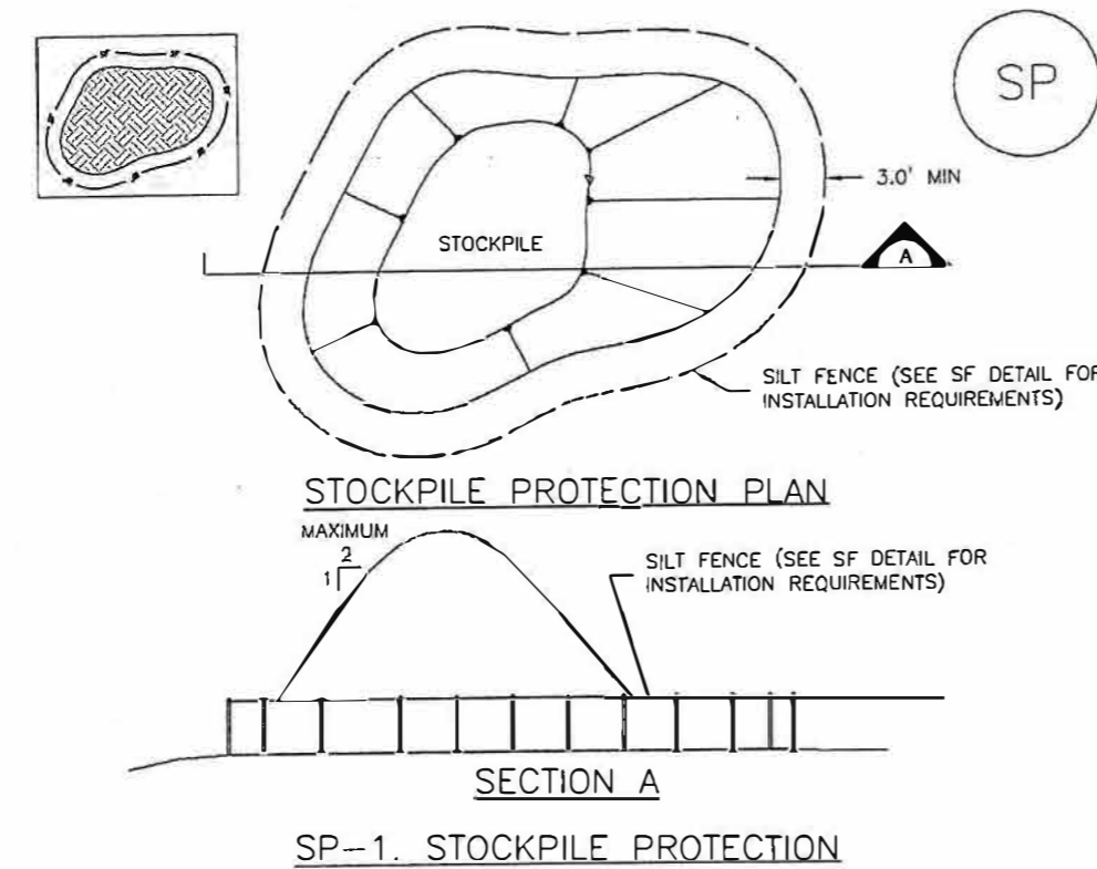
STOCKPILE PROTECTION PLAN
