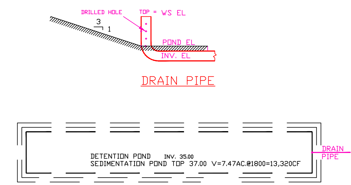
SEDIMENTATION BASINS
