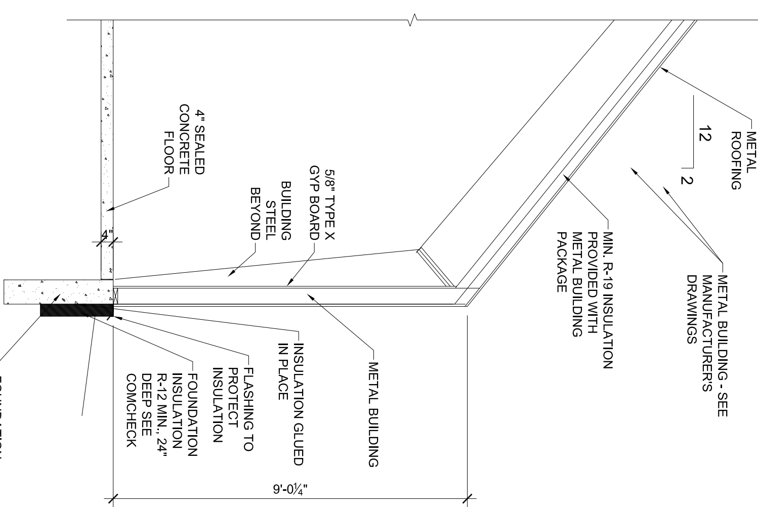
TYPICAL WALL SECTION SCALE: 3/8" = 1'-0" **THIS SECTION TO CHANGE AFTER RECEIVING METAL BUILDING PACKAGE**
