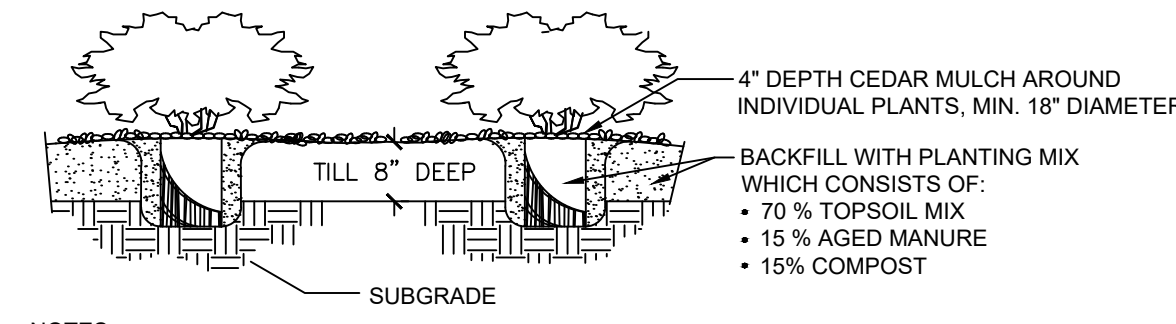
5 SHRUB PLANTING NTS 196-956-011-05
