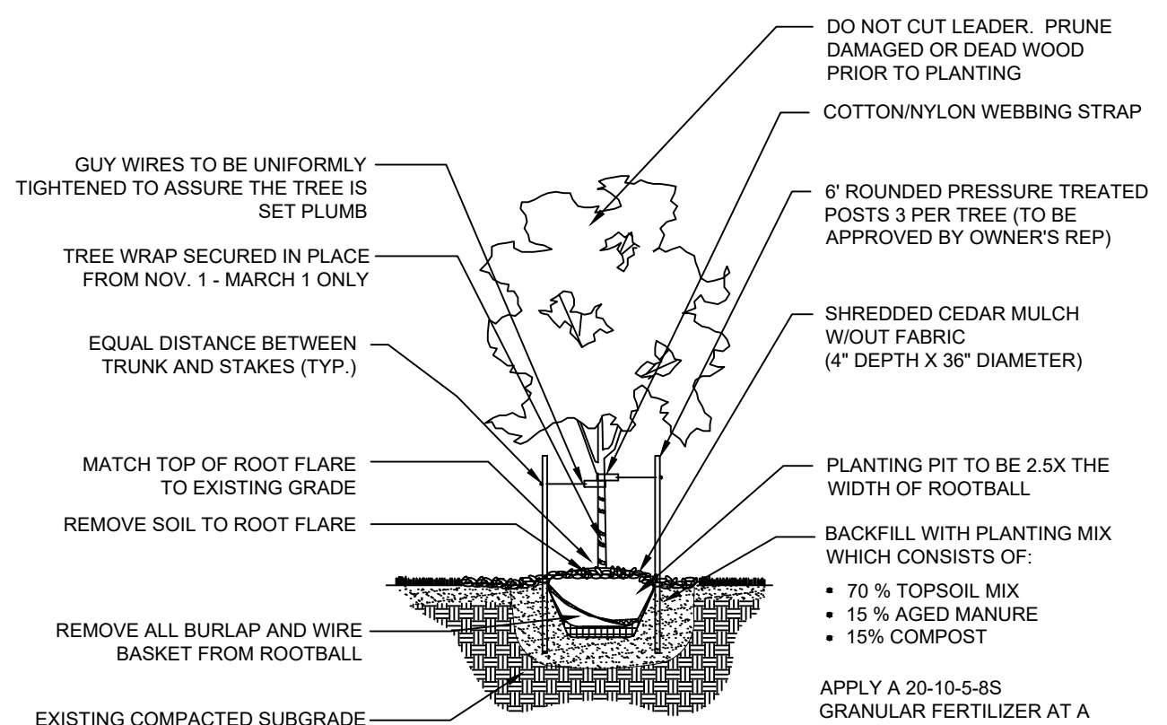
2 DECIDUOUS TREE PLANTING NTS 196-956-011-02
