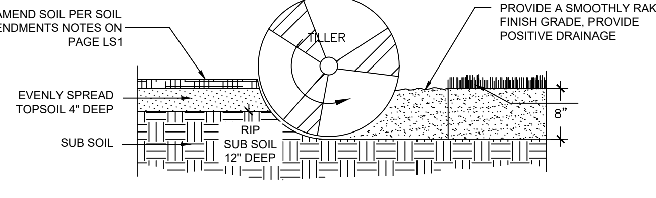
4 SOIL PREPARATION - SOD AREAS NTS 196-956-011-04
