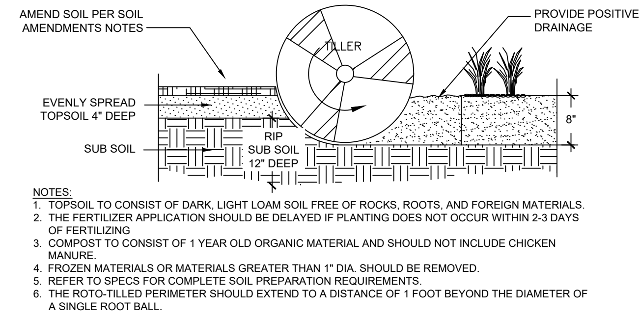
1 SOIL PREP NTS 196-956-011-01
