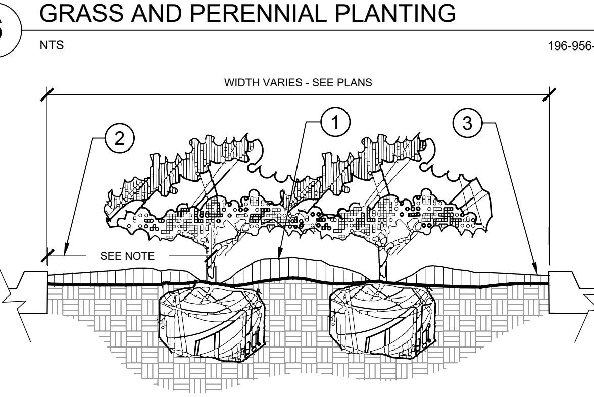
7 PLANTED PARKING LOT ISLANDS/MEDIANS LA-16 SECTION NTS
