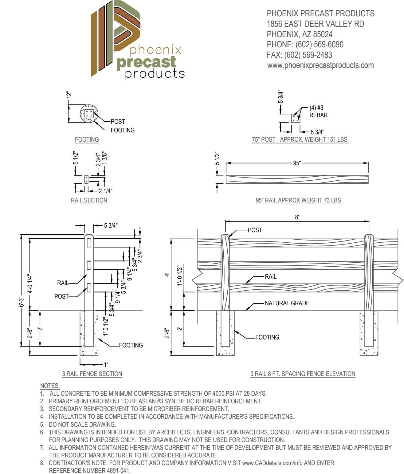
8 3-RAIL SPLIT RAIL FENCE LA-16 1\"/>
