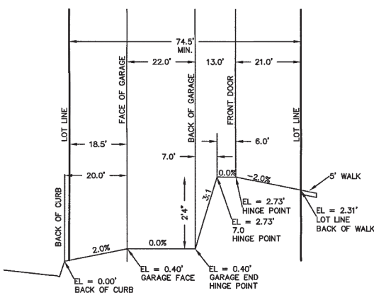
STD-FRONT ENTRY AT GRADE LOT OVERLOT TEMPLATE
