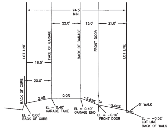
ALT-FRONT ENTRY ELEVATED ABOVE GRADE
