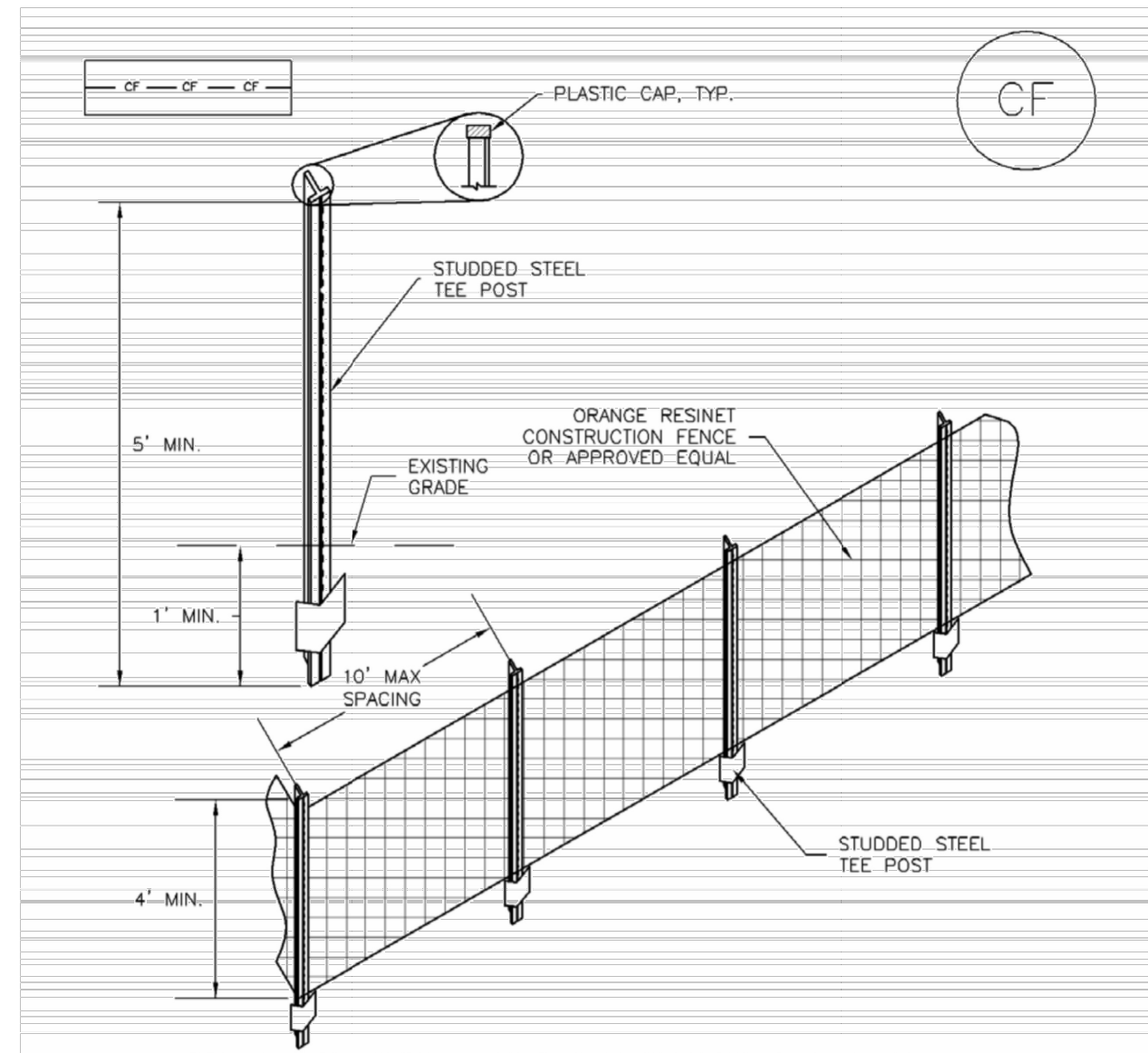
CF-1. PLASTIC MESH CONSTRUCTION FENCE
