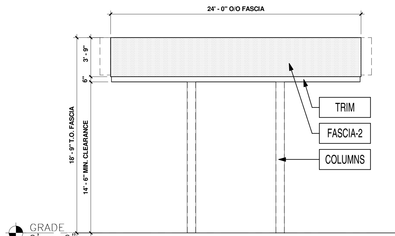
3 WEST ELEVATION 3/16" = 1'-0"
