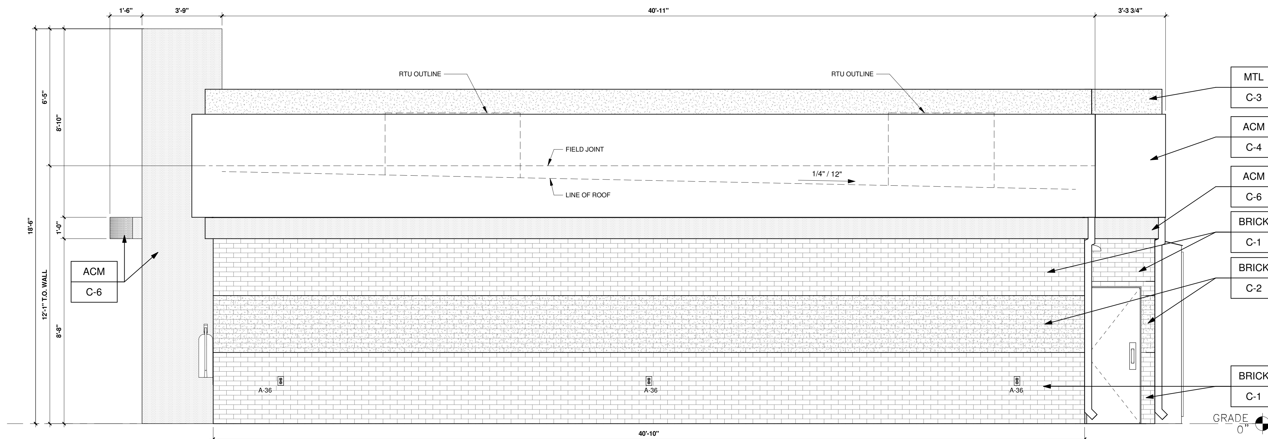
2 WEST ELEVATION 3/8" = 1'-0"
