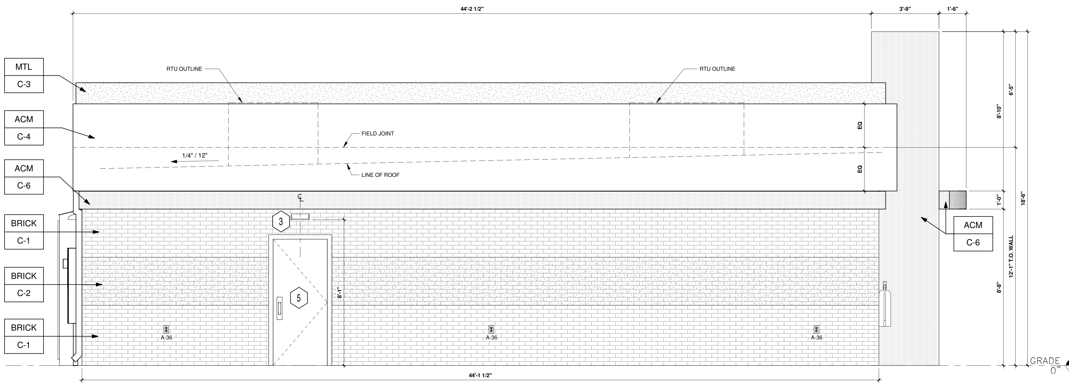
4 EAST ELEVATION - MERIDIAN ROAD 3/8" = 1'-0"
