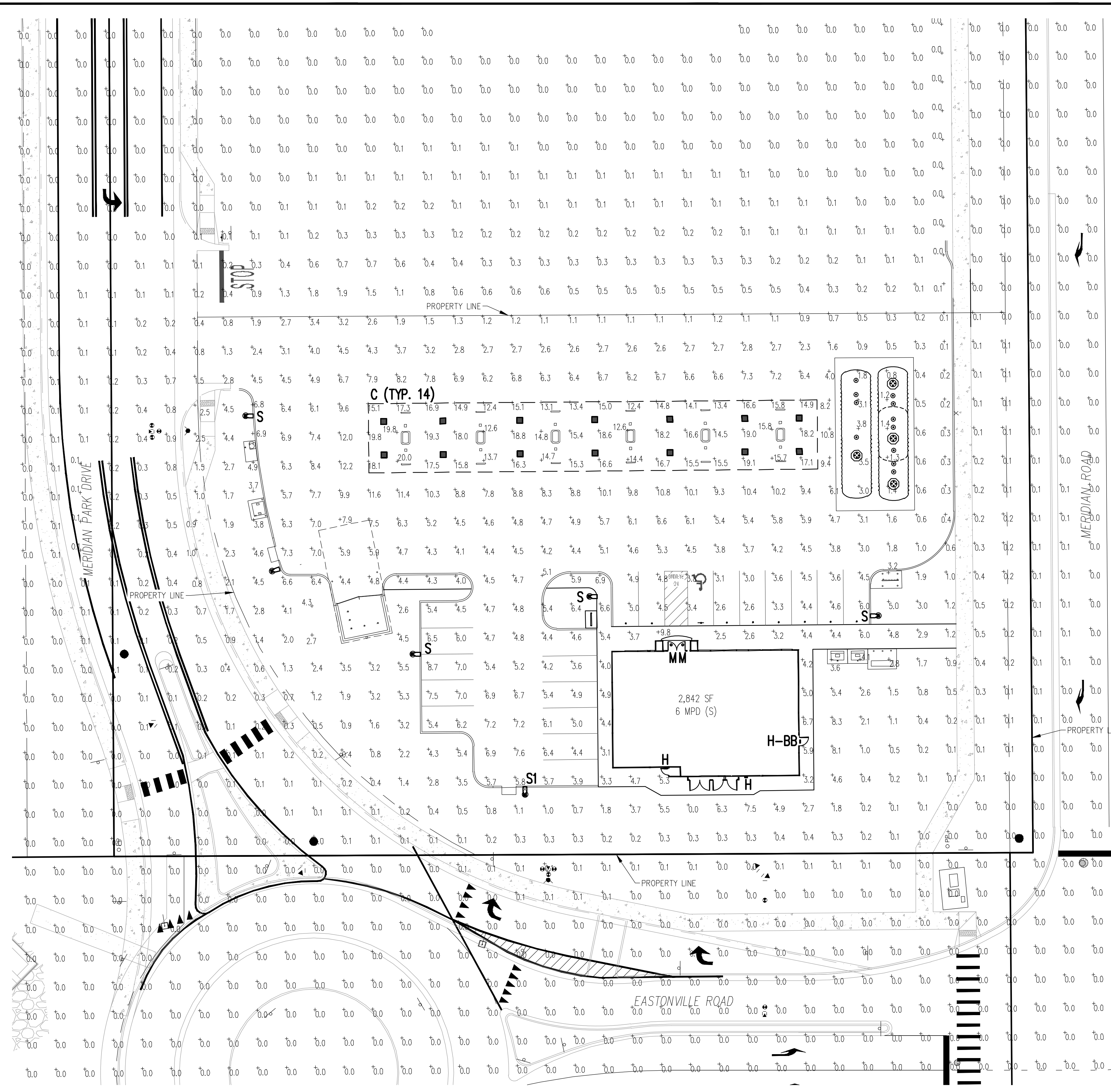
1 PHOTOMETRIC SITE PLAN SCALE: 1"=20'-0"
