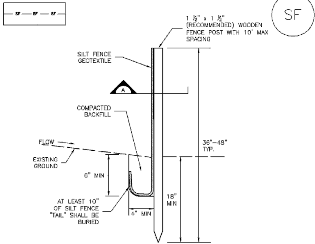
SILT FENCE
