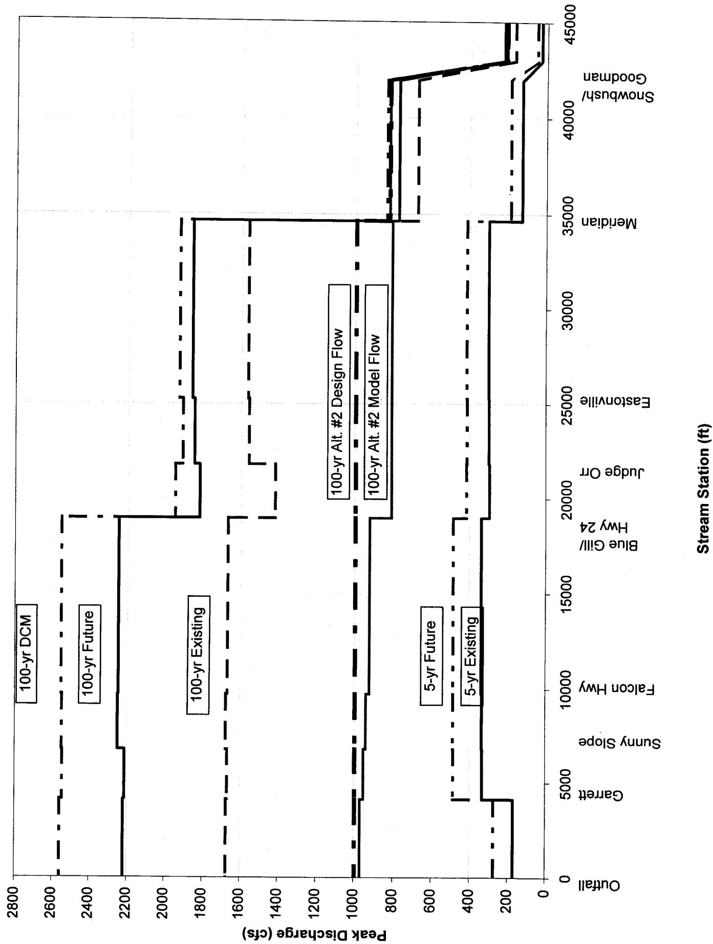
Figure 3-4 HEC-1 Model Results Peak Flows at Major Crossings
