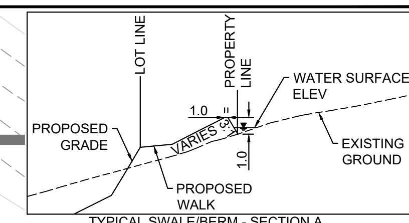
TYPICAL SWALE/BERM - SECTION A NOT TO SCALE
