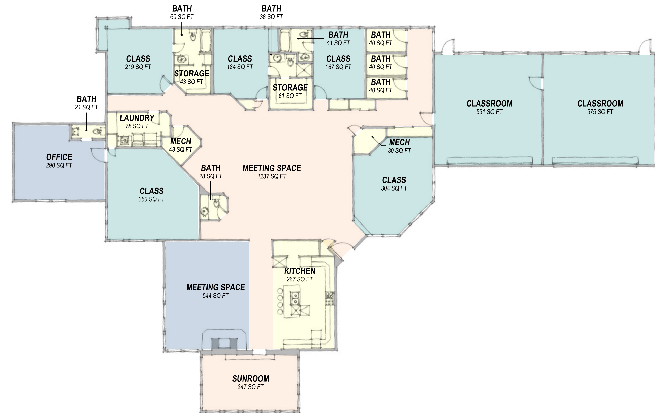
2 SCHOOL HOUSE FLOOR PLAN
