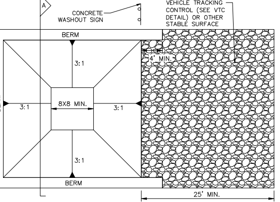
CONCRETE WASHOUT AREA PLAN NTS
