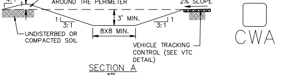
SECTION A NTS
