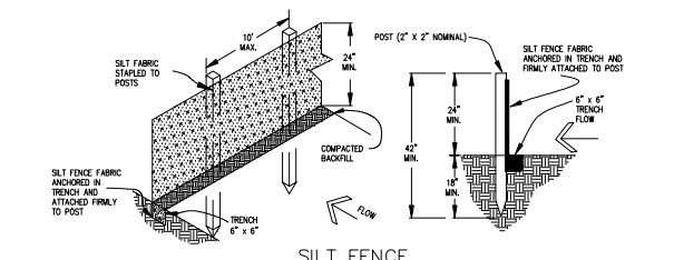
SILT FENCE NTS SILT FENCE NOTES
