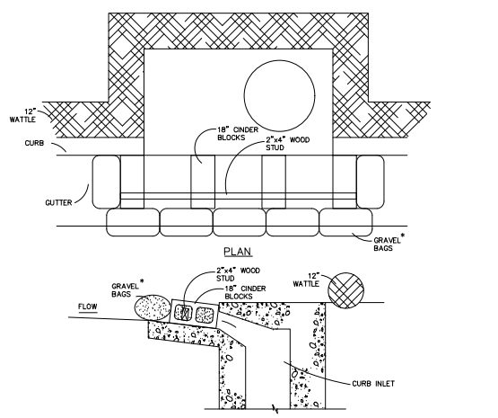
SECTION MODIFIED BLOCK AND GRAVEL BAG CURB INLET PROTECTION NTS
