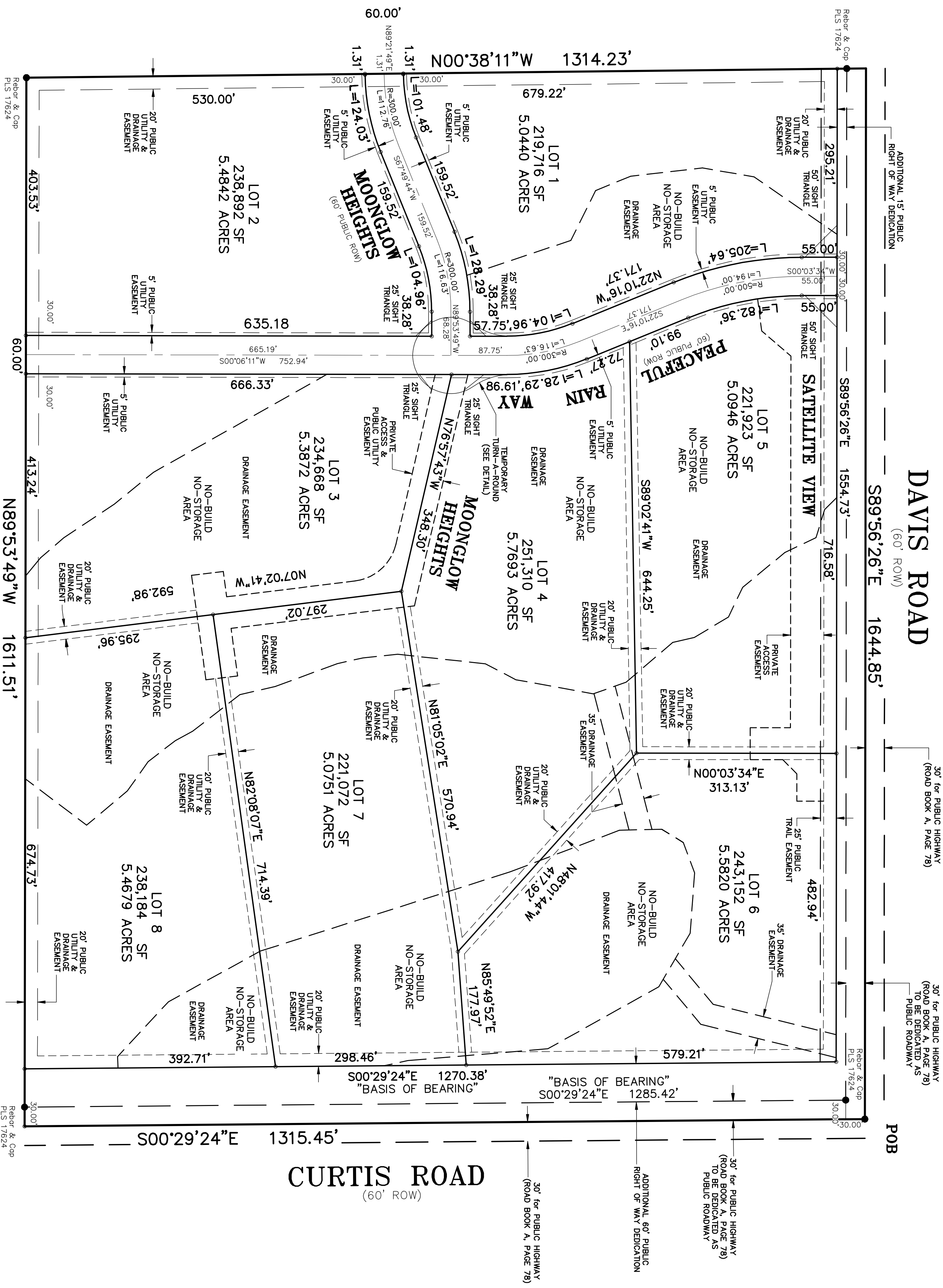
LOT 1 SCALE: 1" = 50'
