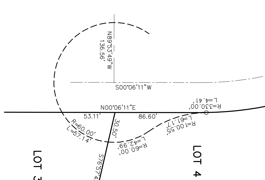
LOT 3 SCALE: 1" = 50'
