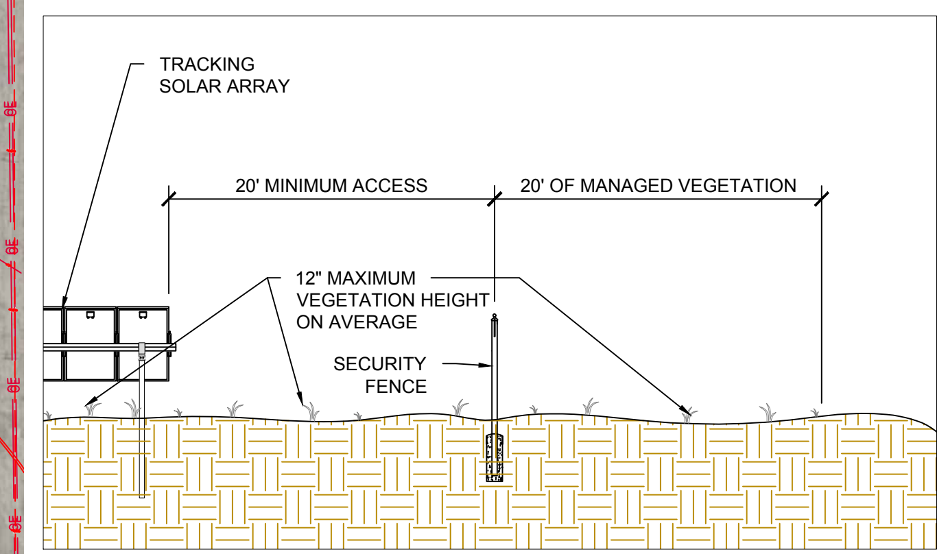
2 SITE PERIMETER ACCESS DETAIL T81 SCALE: NTS
