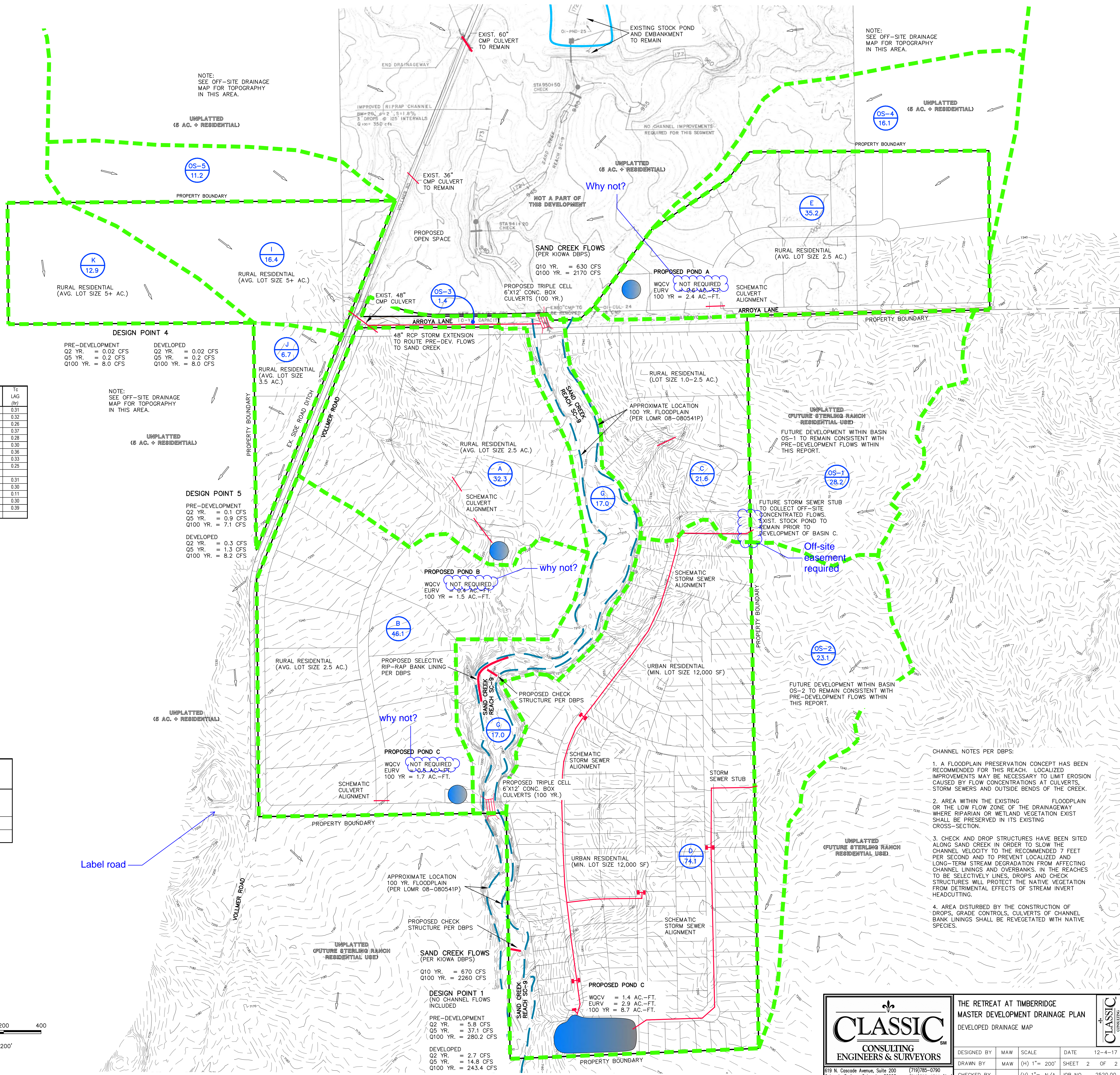
DESIGN POINTS SURFACE ROUTING SUMMARY - DEVELOPED CONDITIONS
