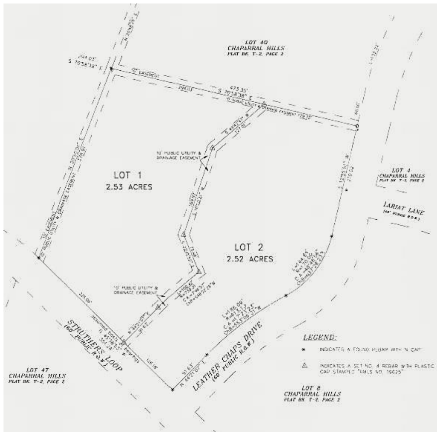
Figure 1-2-2 Proposed Subdivision (not to scale)
