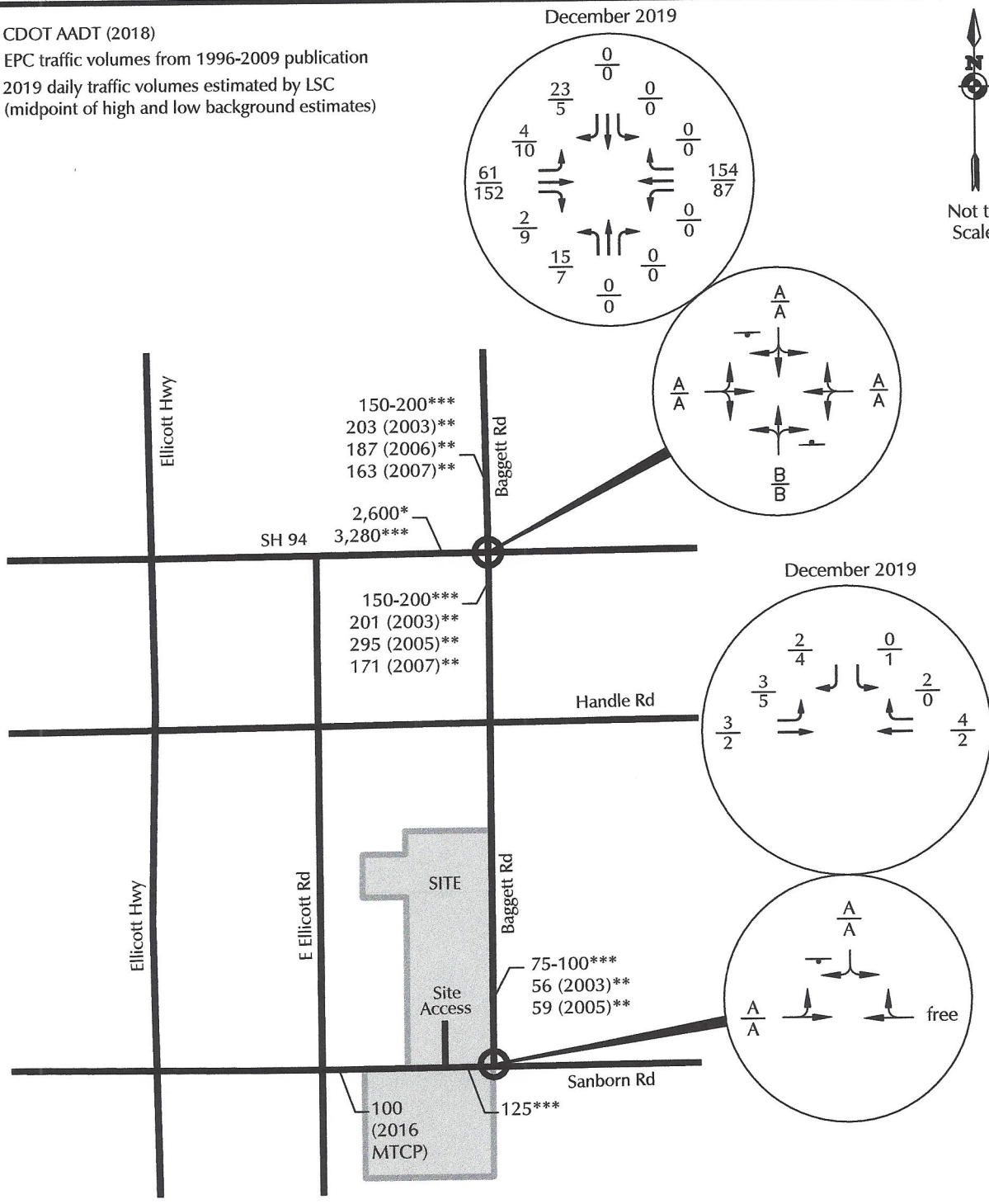
Figure 6 2019 Existing Traffic Volumes, Lane Geometry, Traffic Control, and LOS Ellicott Sand + Gravel (LSC# 194980)
