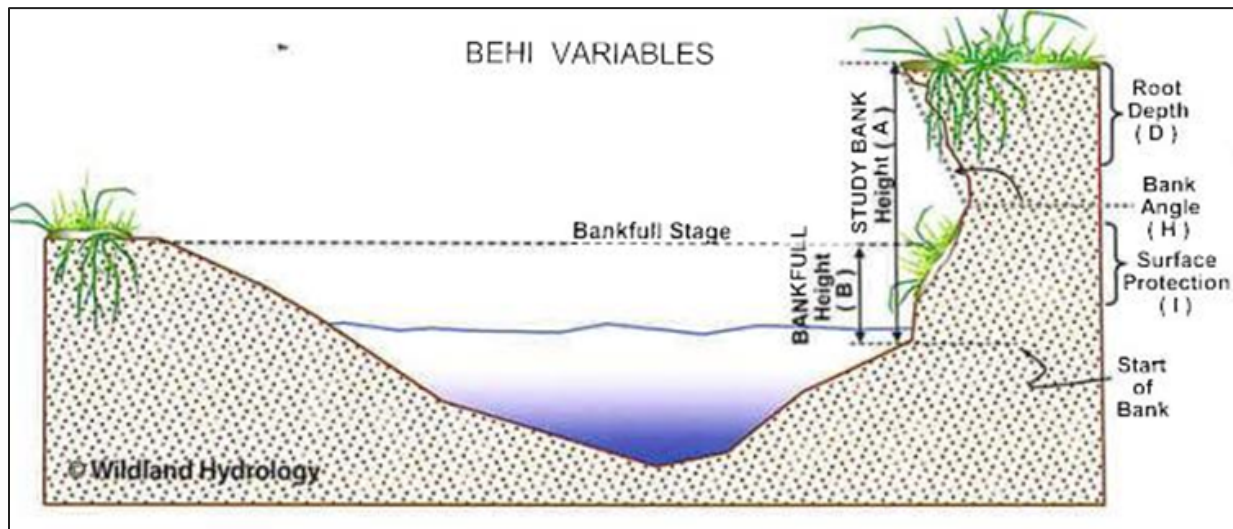
Figure 2-18. BEHI Variables
