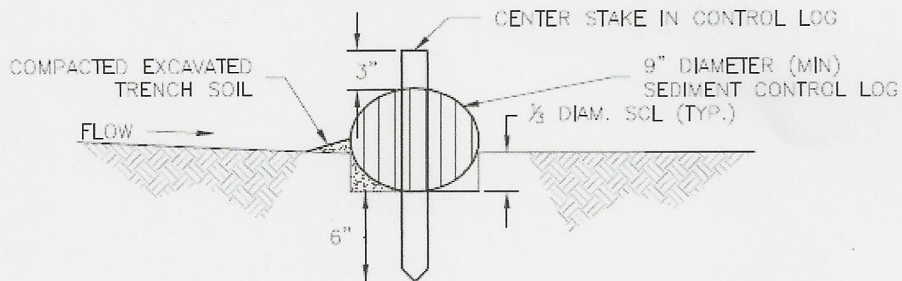
SECTION A TRENCHED SEDIMENT CONTROL LOG (A)
