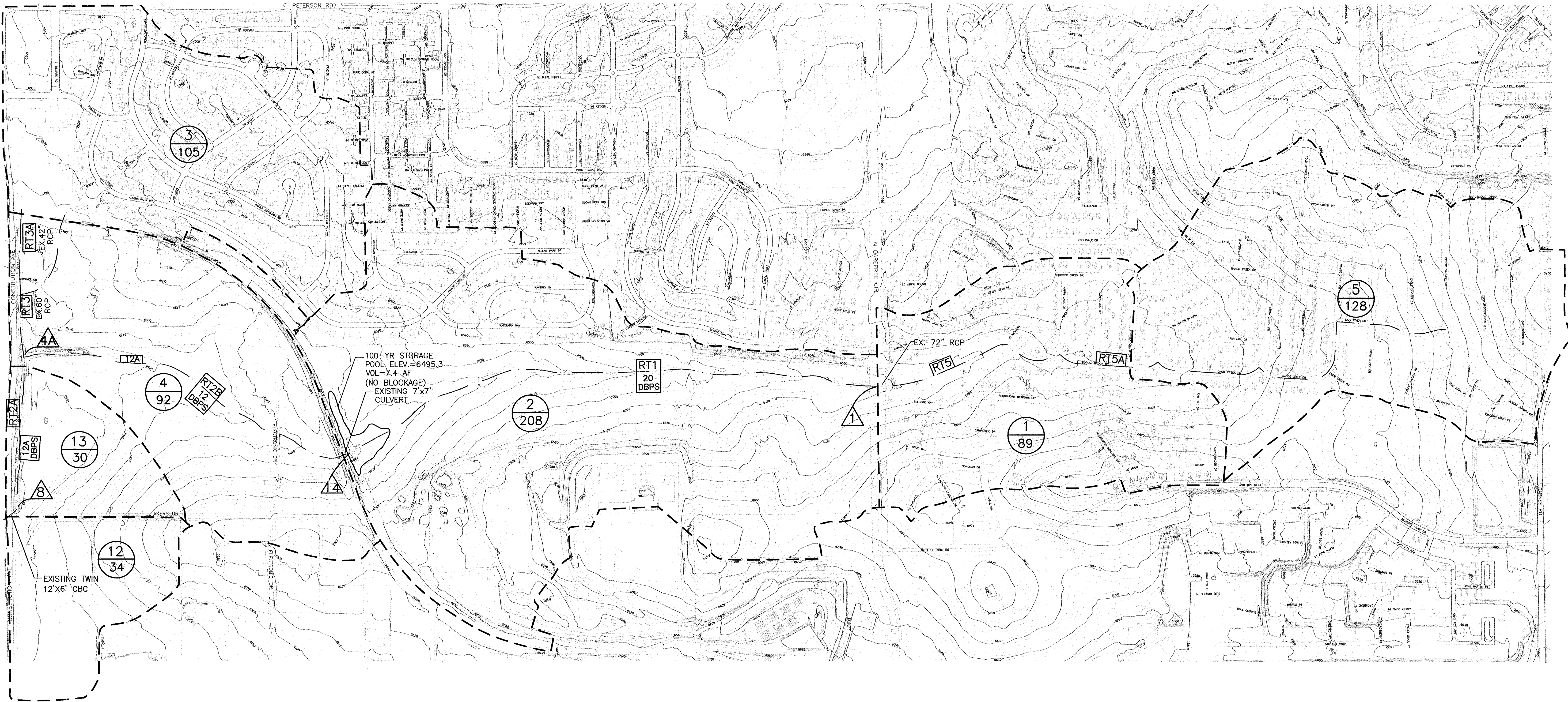
EAST FORK SAND CREEK SUBTRIBUTARY HYDROLOGIC ANALYSIS HYDROLOGIC BASIN MAP EL PASO COUNTY, COLORADO
