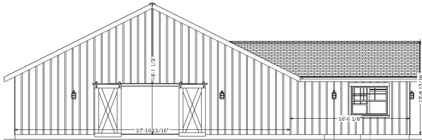
Westside Elevation
