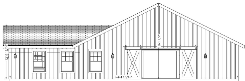
Eastside Elevation
