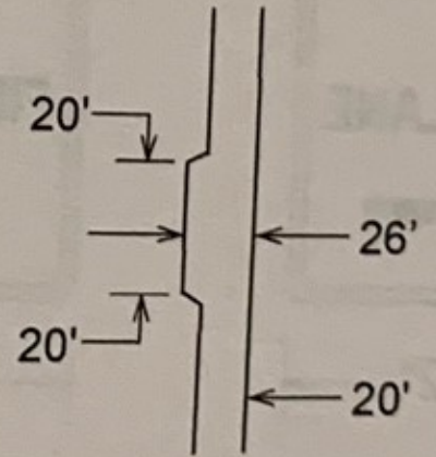
MINIMUM CLEARANCE AROUND A FIRE HYDRANT
