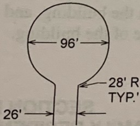
96' DIAMETER CUL-DE-SAC
