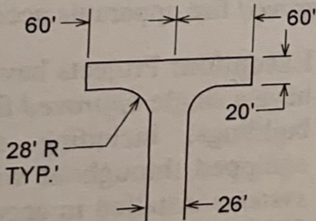
120' HAMMERHEAD
