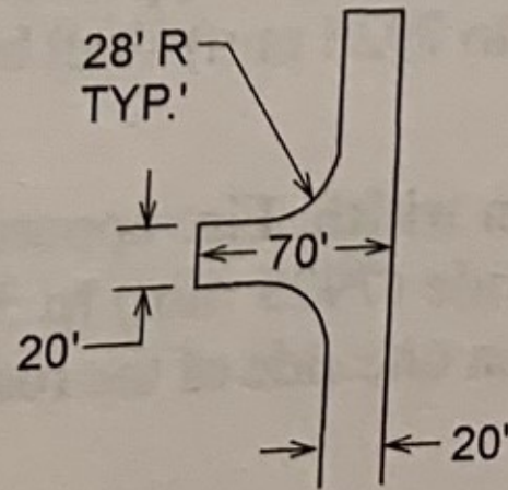
ACCEPTABLE ALTERNATIVE TO 120' HAMMERHEAD
