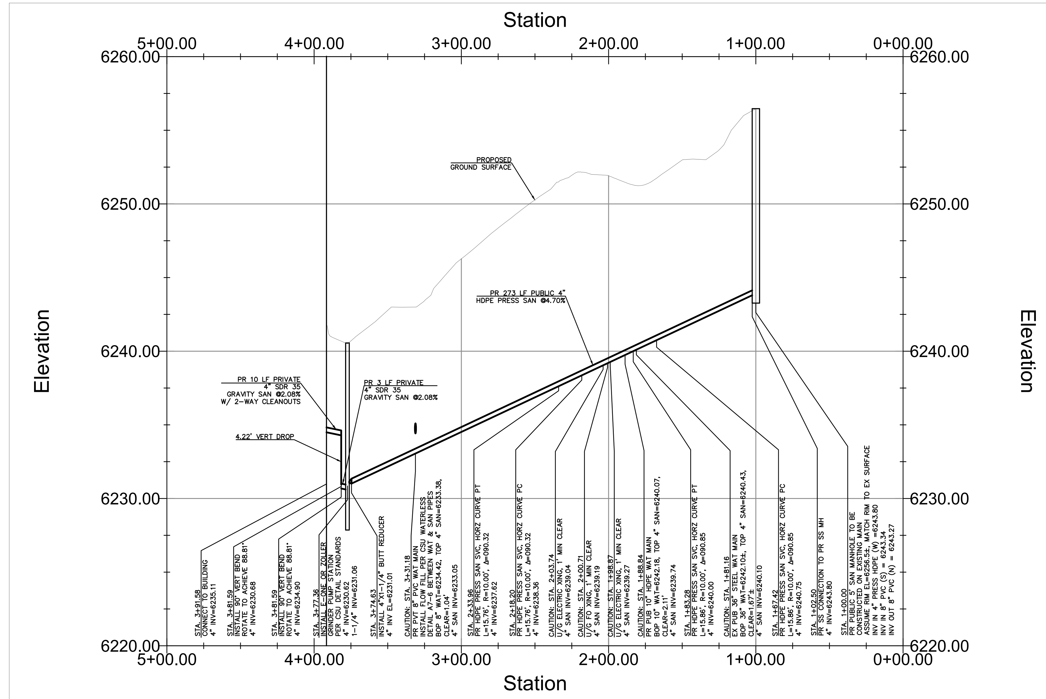
PR WATER MAIN - PROFILE VIEW HORZ SCALE 1" = 40' VERT SCALE 1" = 4'
