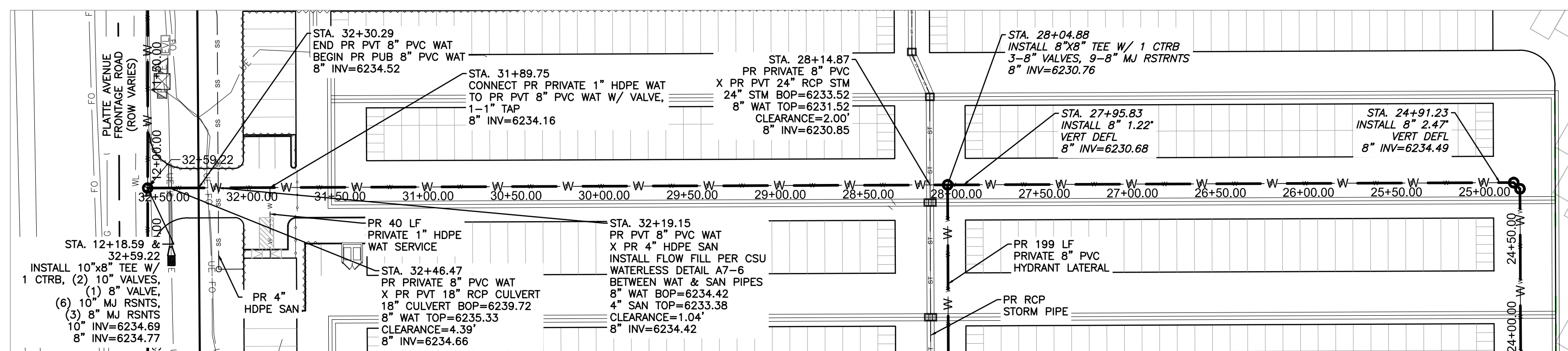
PR WATER MAIN - PLAN VIEW
