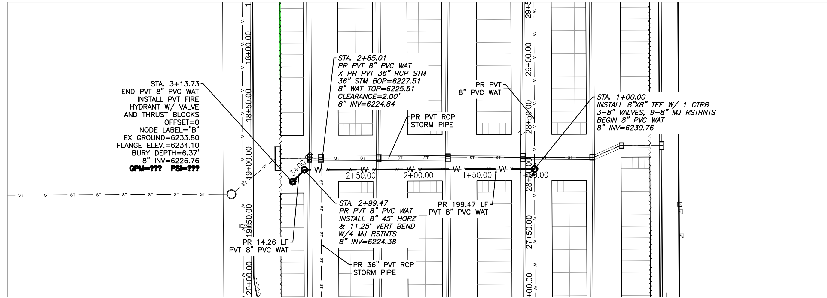
PR HYDRANT LATERAL – PLAN VIEW
