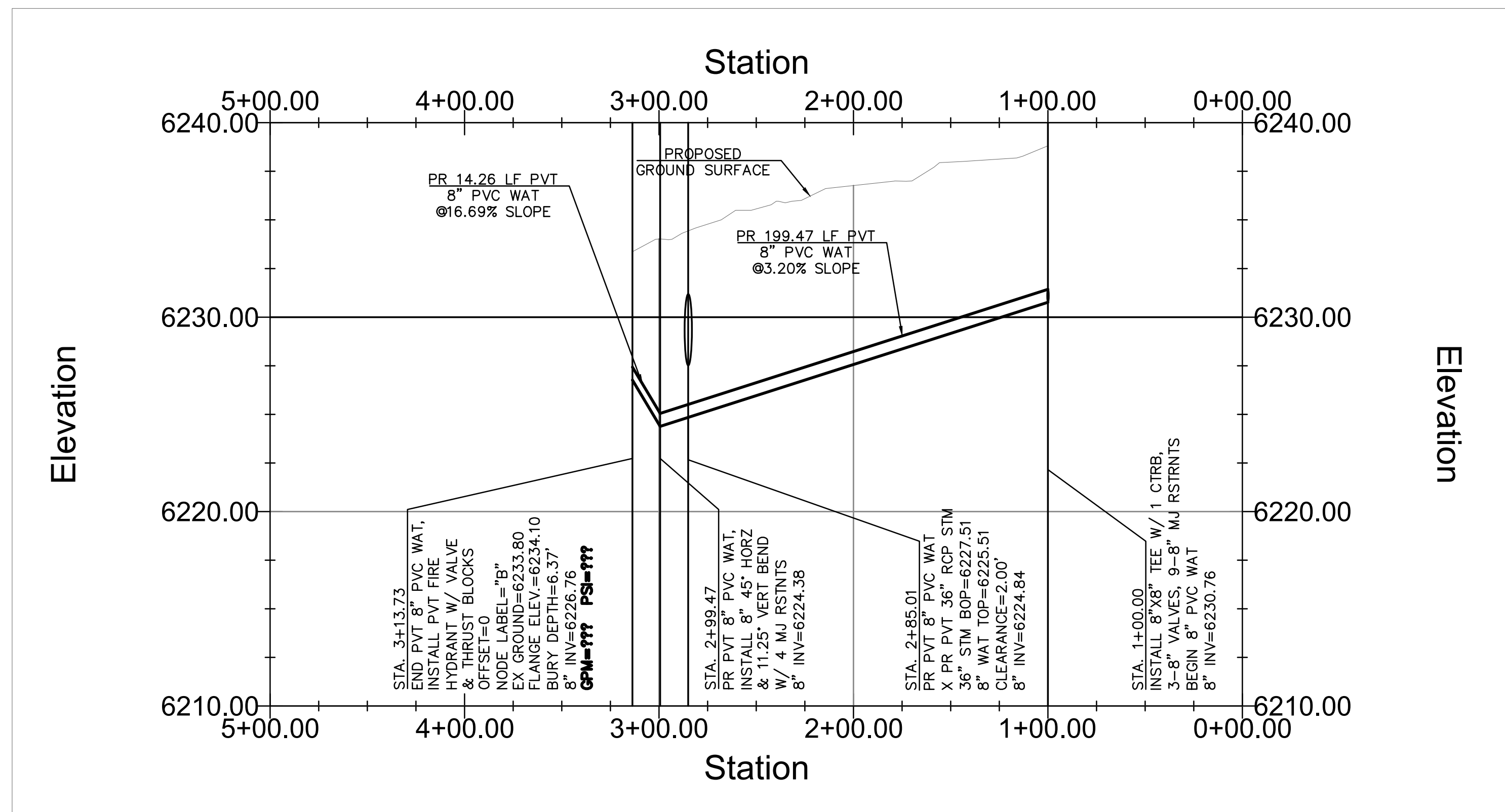
PR HYDRANT LATERAL – PROFILE VIEW
