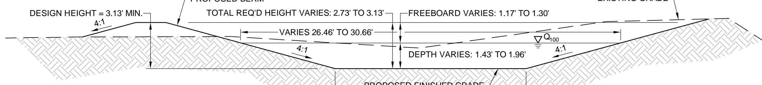
DRAINAGE CHANNEL (B) NOT TO SCALE
