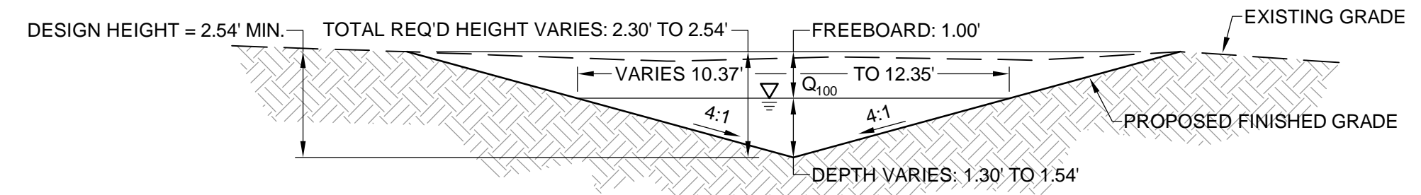
DRAINAGE SWALE (A) NOT TO SCALE
