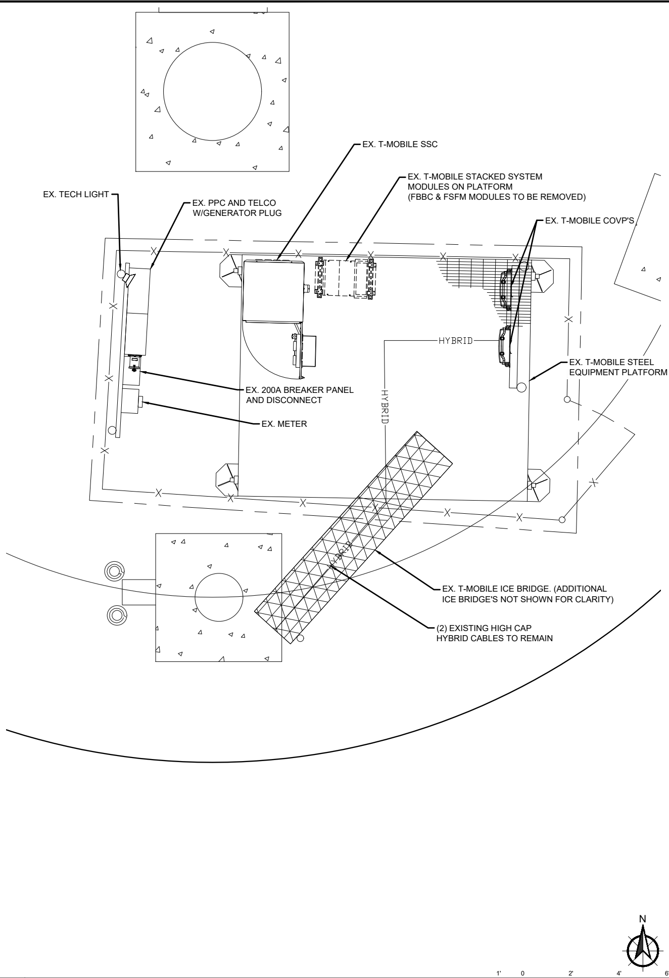
1 EXISTING EQUIPMENT LAYOUT SCALE: 1/2" = 1'-0"
