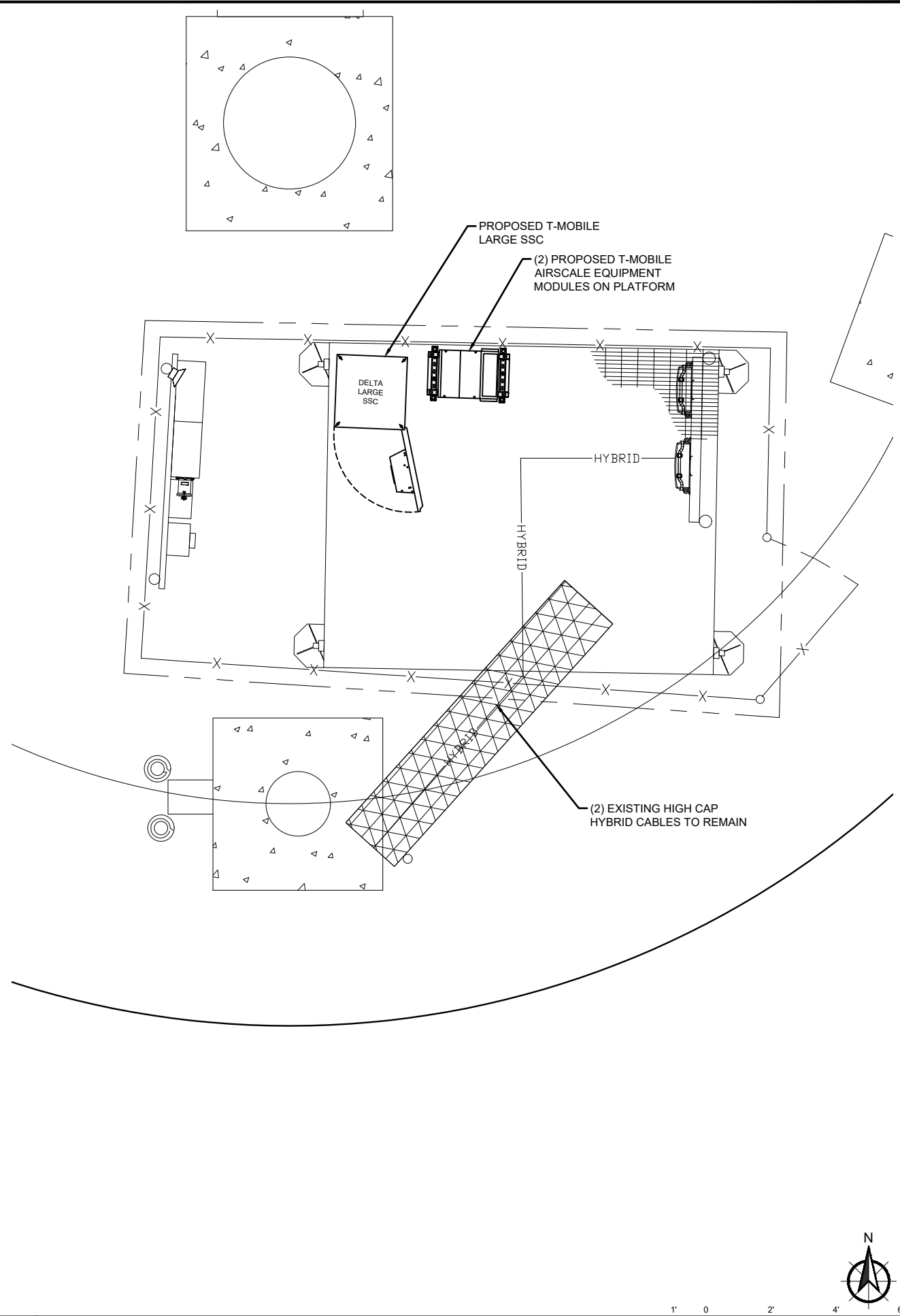
2 PROPOSED EQUIPMENT LAYOUT SCALE: 1/2" = 1'-0"
