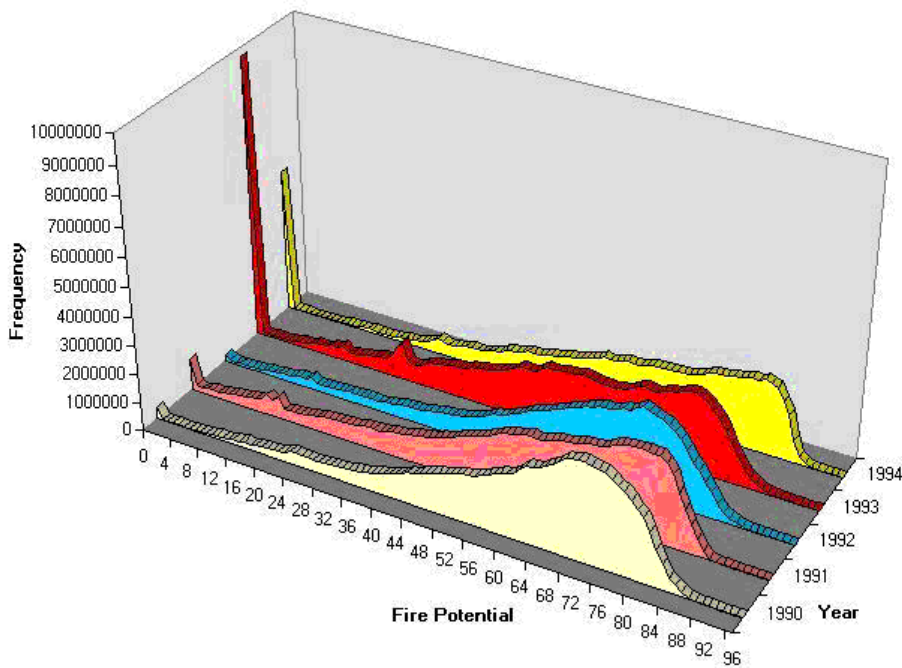
Figure 8. The frequency of pixels in the entire study area is shown for Fire Potential Index values calculated for 1990 to 1994.
