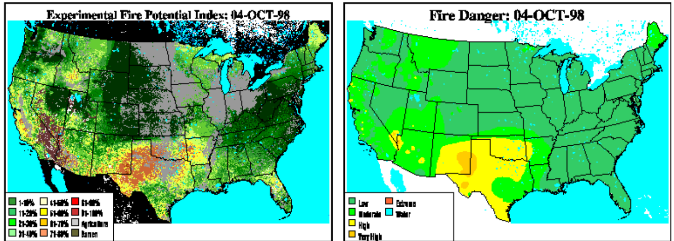
Figure 6b. The standard NFDRS map is provided for comparison with the fire potential index map ( http://www.fs.fed.us/land/wfas/exp_fp_4.gif ).
