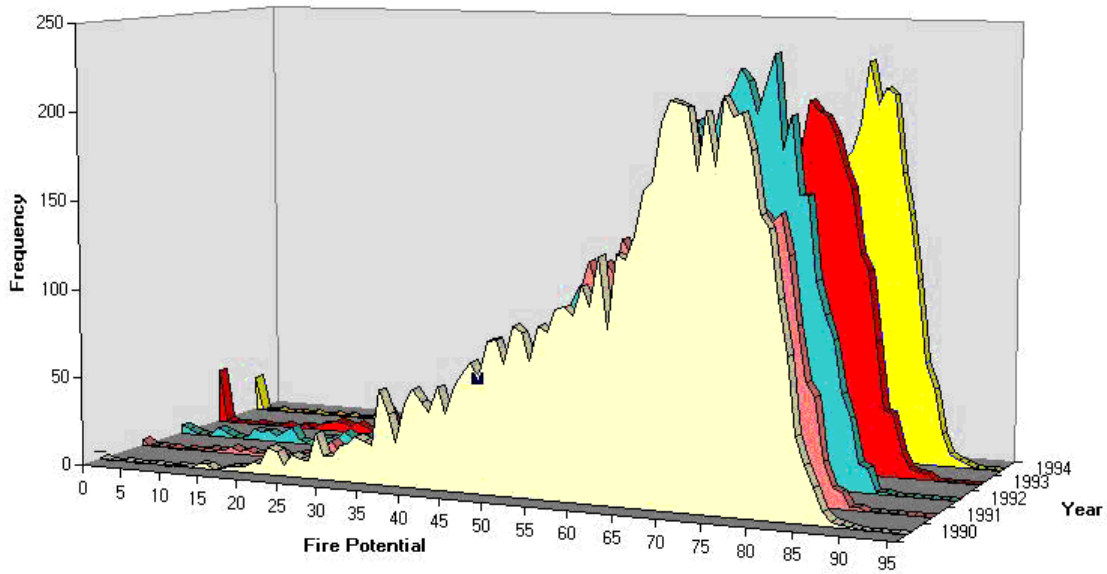
Figure 7. For only those pixels in which fires occurred, in the years 1990 to 1994, the frequency of FPI index values is shown.
