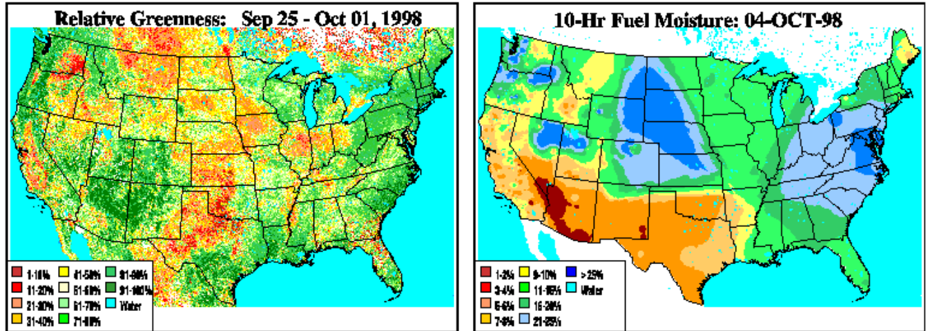
Figure 6a. Relative greenness, 10-hour fuel moisture maps, and NFDR fuel model (fig. 4) and the maximum live ratio (fig.5) maps are inputs to the FPI map calculation.
