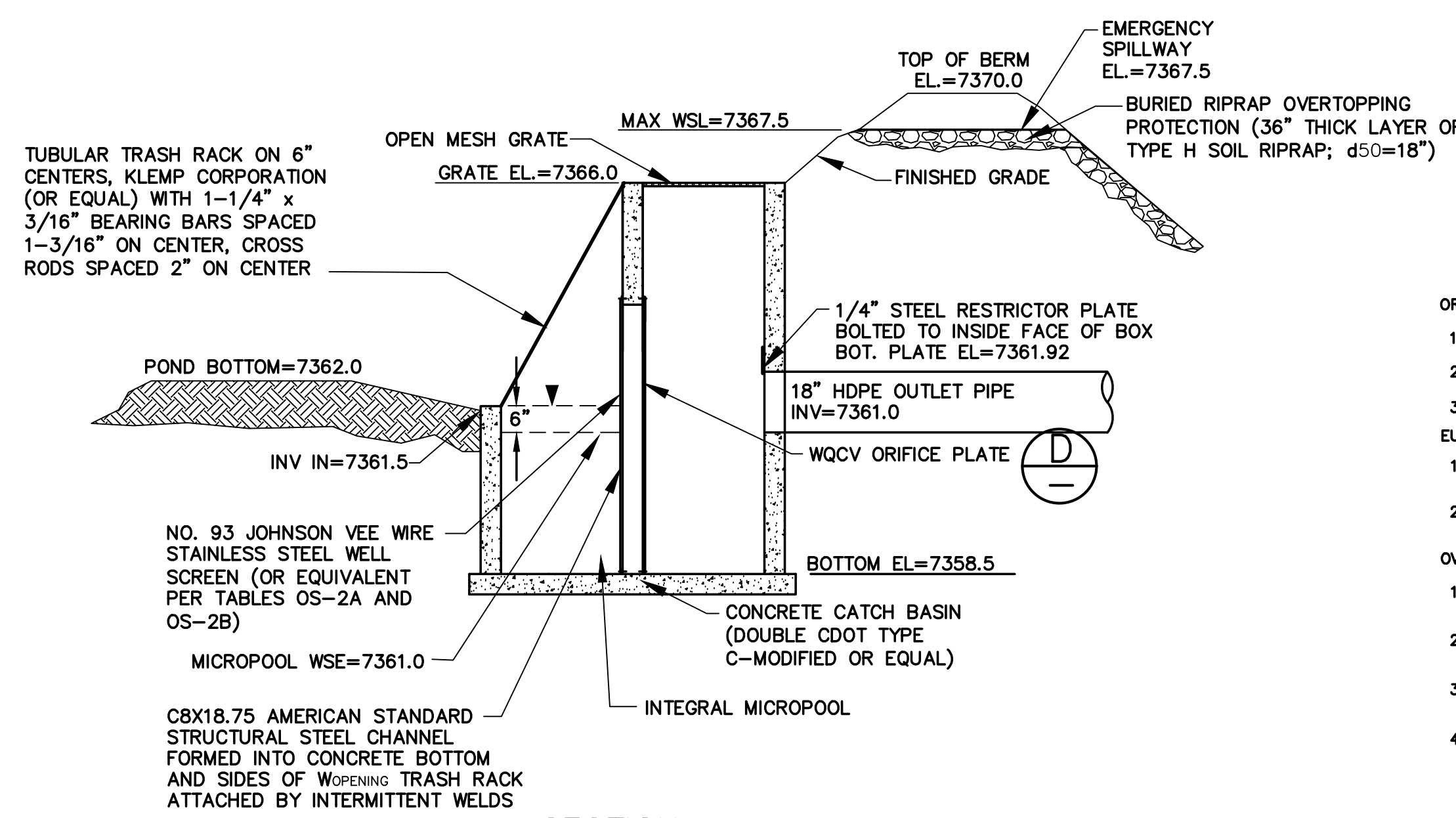
SECTION C DETENTION POND OUTLET STRUCTURE C SCALE: NTS
