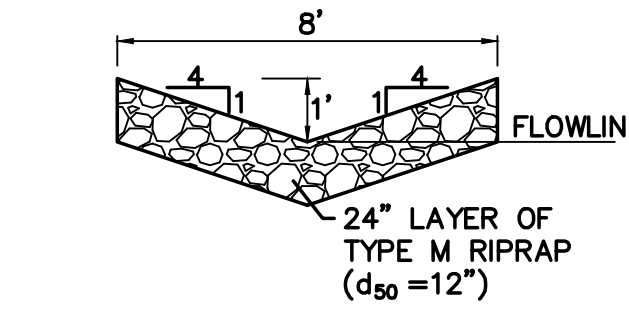
RIPRAP RUNDOWN E NOT TO SCALE
