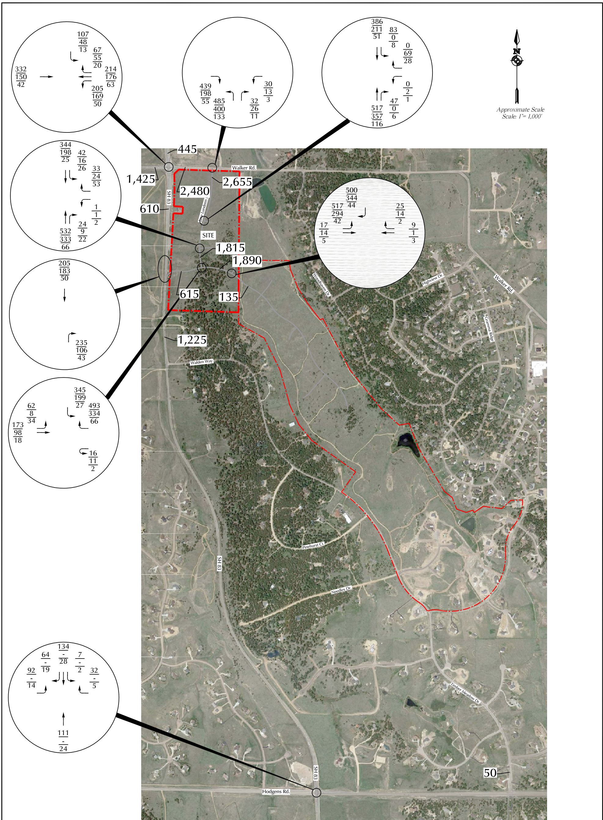
Figure 14 Long-Term Assignment of Phase 1 and 2 Site-Generated Traffic Monument Academy (LSC #184820)
