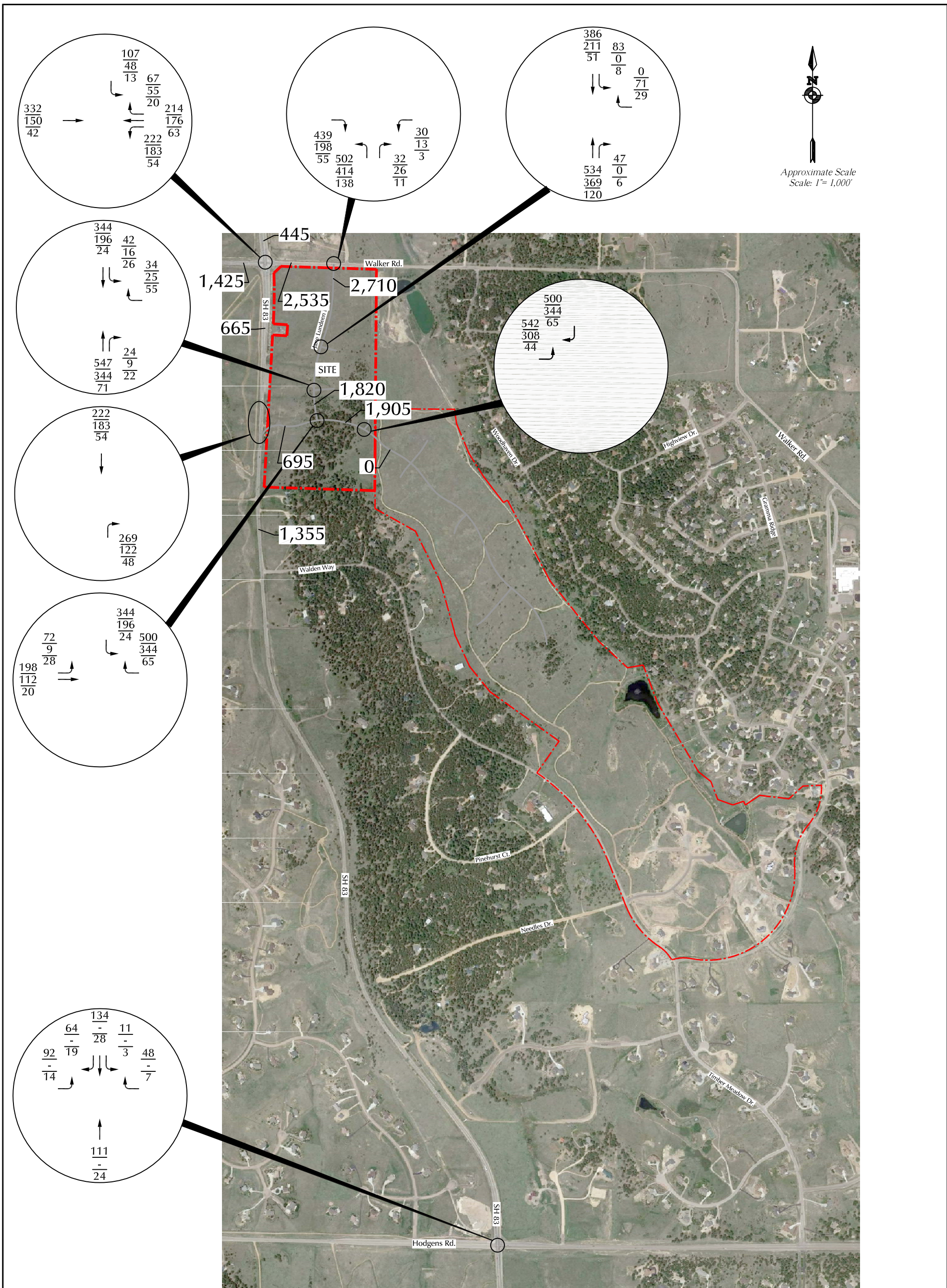
Figure 13 Short-Term Assignment of Phases 1 and 2 Site-Generated Traffic Monument Academy (LSC #184820)
