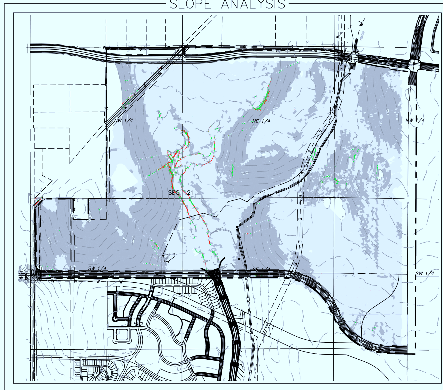
SLOPE ANALYSIS
