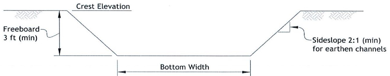
Spillway Section
