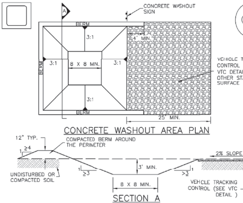
CWA-1. CONCRETE WASHOUT AREA
