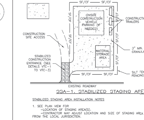
SSA-1. STABILIZED STAGING AREA
