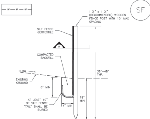
SILT FENCE
