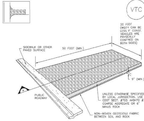
VTC-1. AGGREGATE VEHICLE TRACKING CONTROL
