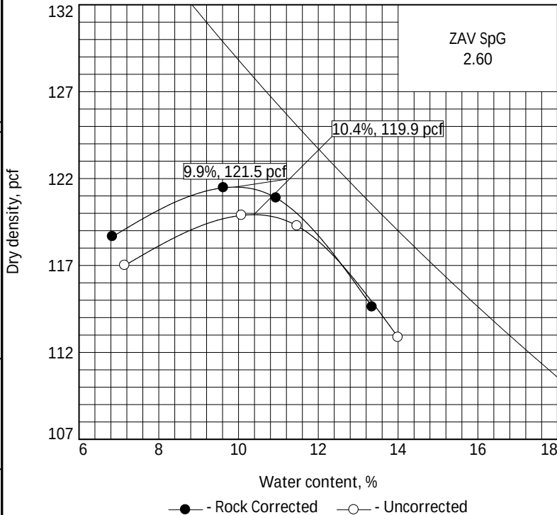
COMPACTION TESTING DATA AASHTO T 99-22 Method A Standard AASHTO T 99/T 180 Annex A Oversize Corr. Applied to Each Test Point
