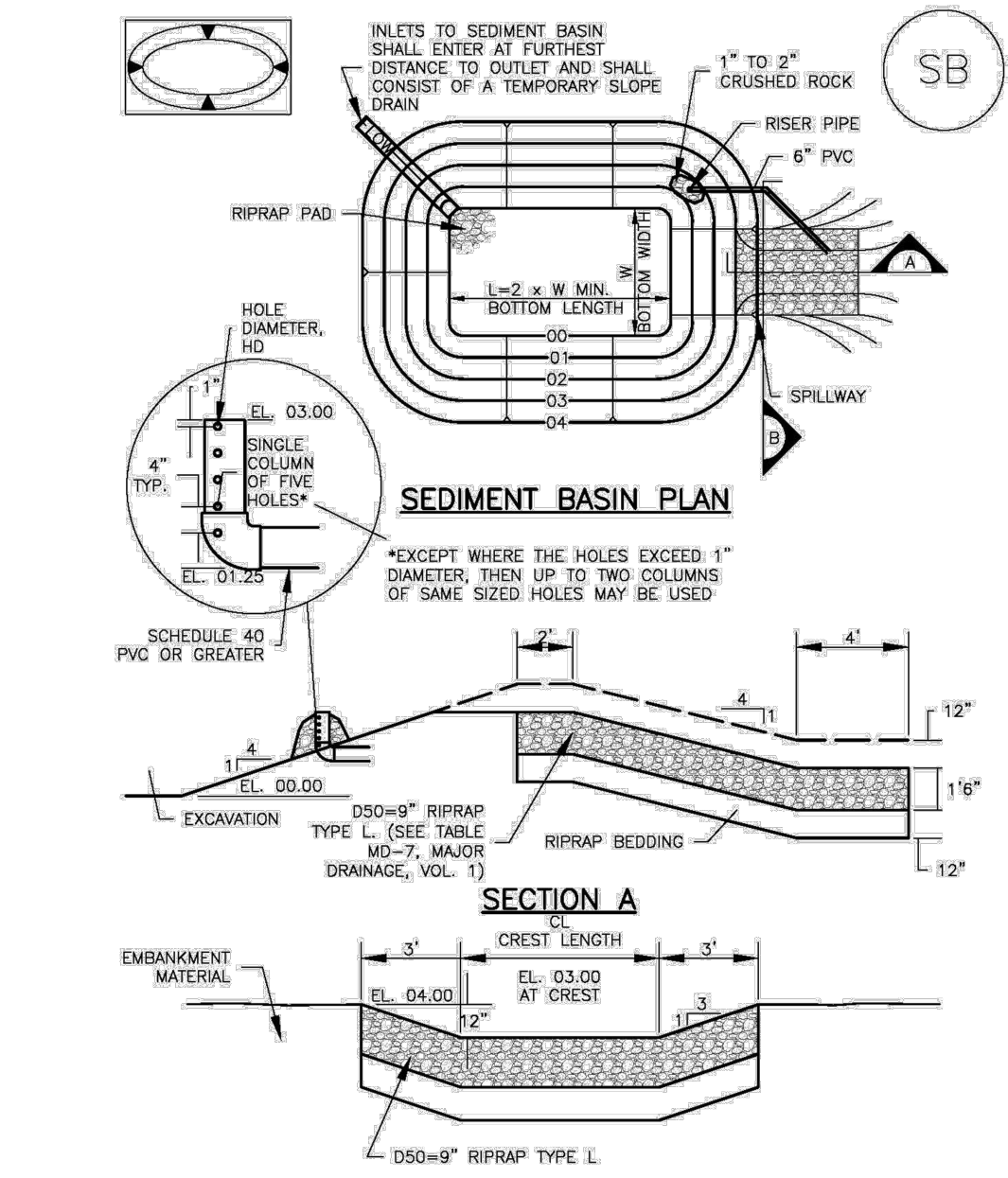
SB-1. SEDIMENT BASIN PLAN
