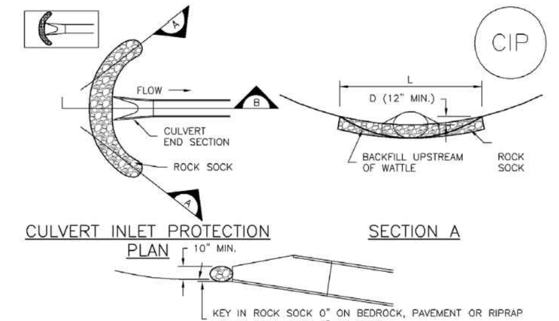
CIP-1. CULVERT INLET PROTECTION
