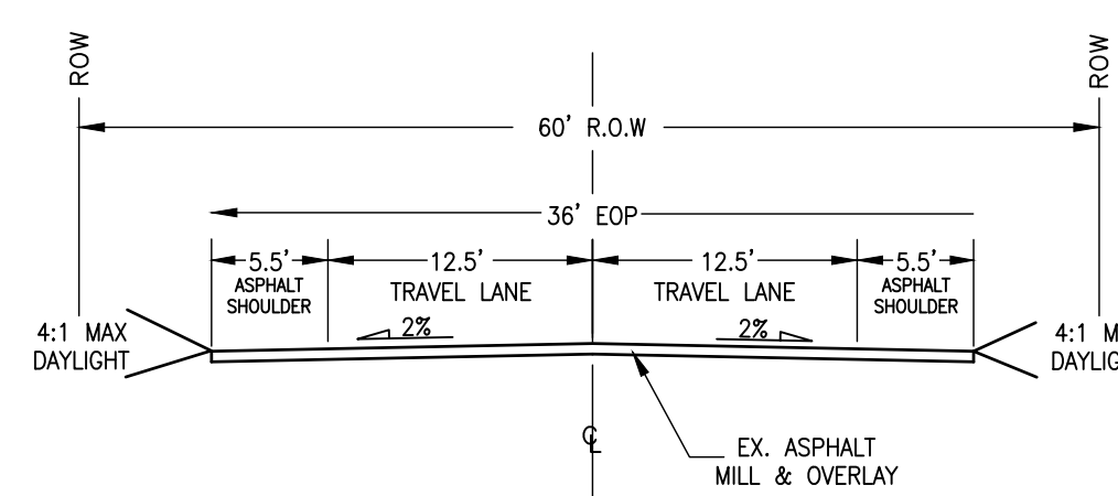
VOLLMER ROAD INTERIM CROSS SECTION SCALE: NTS
