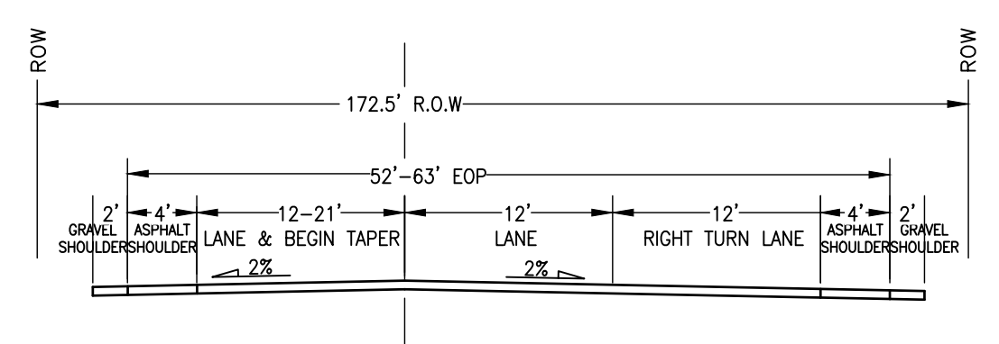
VOLLMER ROAD INTERIM CROSS SECTION SCALE: NTS
