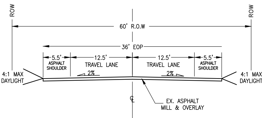
VOLLER ROAD INTERIM CROSS SECTION SCALE: NTS
