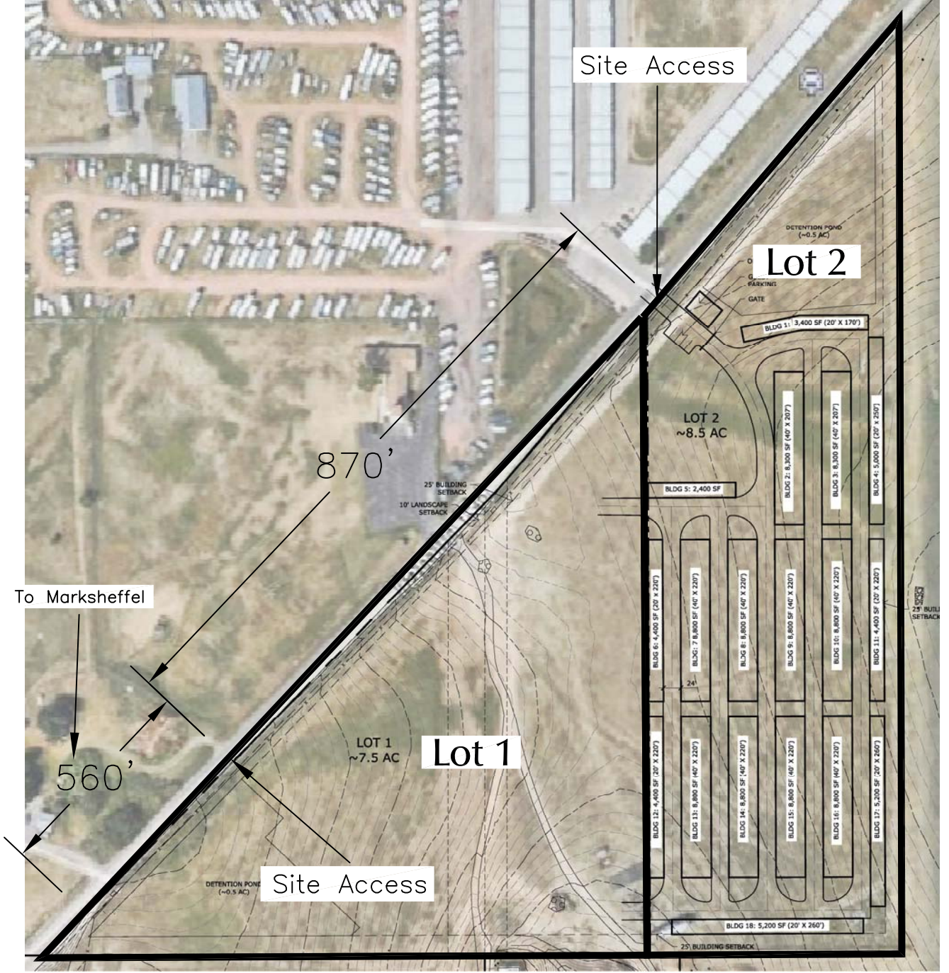
Figure 2 Site Plan Tamlin Rd. Rezone (LSC# 184610)
